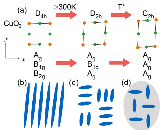
FIG. 5. (Color online) (a) The reduction of symmetries consistent with the observed polarization anisotropy. The CuO 2 layers are shown. Using the centrosymmetric refinement [39], the highest possible symmetry below T^* is C_{2h} . The relevant irreducible representations are given in each case. (b) Schematic representations corresponding to nematic ordering, (c) short stripe ordering [41–46], and (d) local polaronic order [47].
