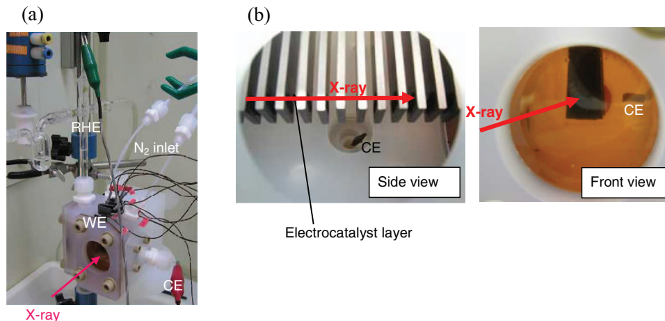
FIG. 3. Photographs of the spectroelectrochemical cell. (a) Overall view: The cell in the experimental hutch. Red and green clips were connected to the CE and RHE, respectively. Other wires were connected to the WE. X-rays entered from the left side, as indicated by the arrow. (b) Inside view of the cell; left: side view, right: front view.
