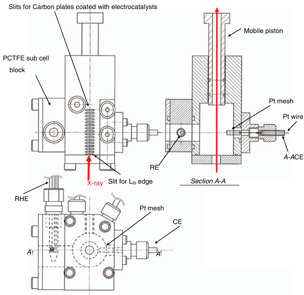
FIG. 2. Schematic diagram of the spectroelectrochemical cell.
