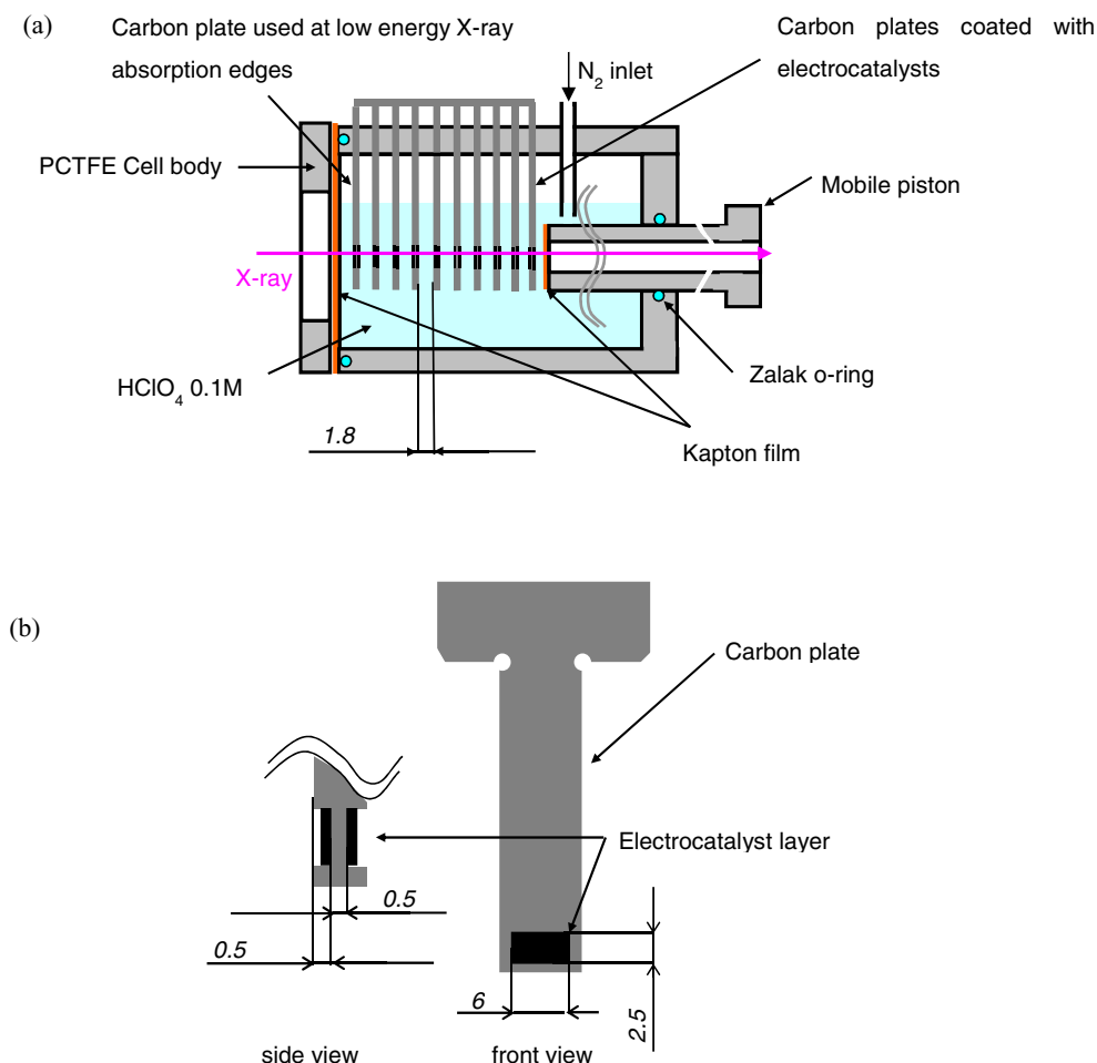
FIG. 1. Schematic diagrams of the spectroelectrochemical cell. (a) Sectional drawing of the cell and (b) magnified diagram of the carbon plate coated with electrocatalyst (black areas) on both sides of the recesses in the carbon plate.
