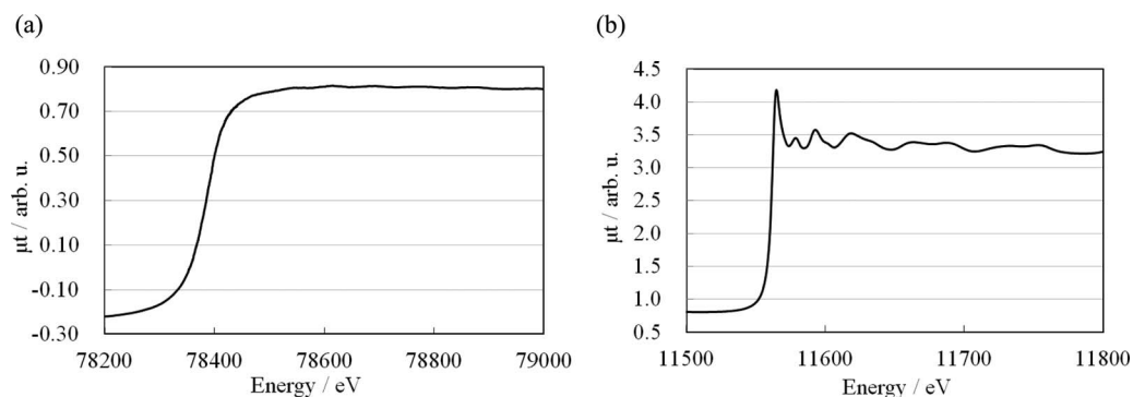
FIG. 6. XAFS spectra of Pt foil. (a) Pt K-edge and (b) Pt L_{III} -edge.
