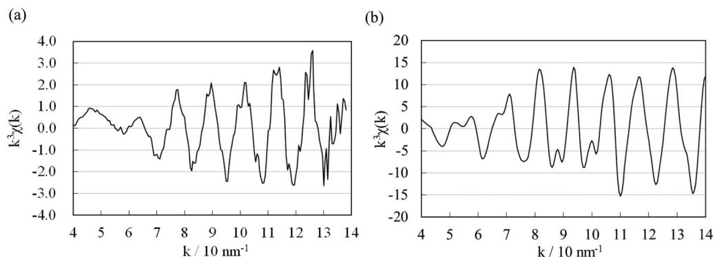
FIG. 7. XAFS oscillations of Pt foil. (a) Pt K-edge and (b) Pt L_{III} -edge.
