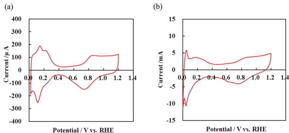
FIG. 5. CVs of the Pt/C electrocatalyst. (a) RDE and (b) spectroelectrochemical cell.
