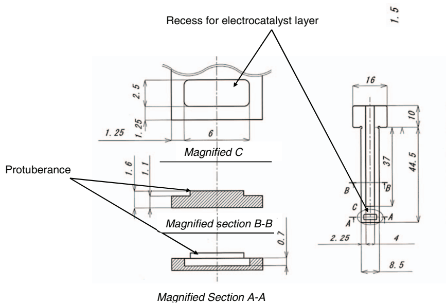
FIG. 4. Diagram of the carbon plate used for L-edge experiments. An electrocatalyst layer is formed on one side of the plate.
