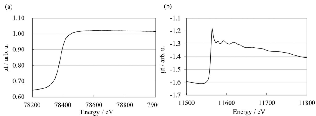
FIG. 8. In situ X-ray absorption spectra of Pt/C at 0.4 V vs. RHE. (a) Pt K-edge and (b) Pt L III -edge.
