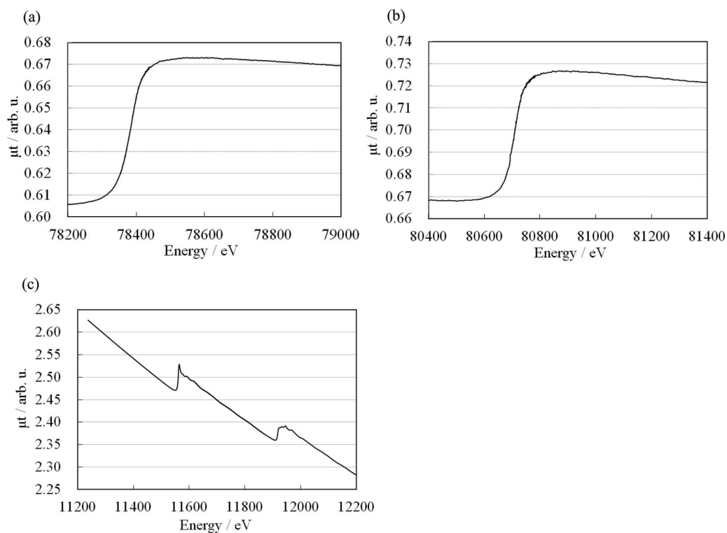
FIG. 10. In situ XAFS spectra of Pt/Au/C at 0.4 V vs. RHE; (a) Pt K-edge, (b) Au K-edge and (c) Pt and Au L III -edges.
