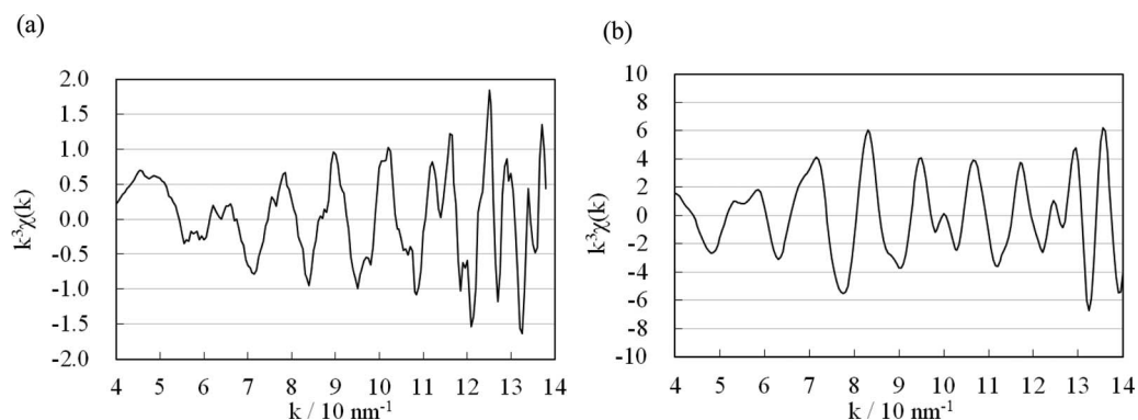
FIG. 9. XAFS oscillations of Pt/C at 0.4 V vs. RHE; (a) Pt K-edge and (b) Pt L III -edge. Reproduced with permission from Kaito et al. , J. Phys. Chem. C 118 (16), 8481–8490 (2014). Copyright 2014 by the American Chemical Society.
