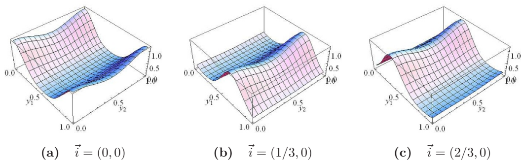
Figure 1. The probability densities of zero-mode wavefunctions |\Theta^{\vec{i}, \mathbb{N}}(\vec{z})|^2 on (y_1, y_2) -plane for Type 1, where we set (x_1, x_2) = (0, 0) . These figures show that the peaks of the probability densities are located at \vec{y} = -\vec{i} .
