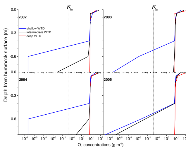
Fig. 11. Vertical profile distributions of peat soil aqueous oxygen concentrations ( [O_{2s}] ) simulated under hummock surface during shallow (DOY 15, 55, 25 and 55 of 2002, 2003, 2004 and 2005 respectively), intermediate (DOY 135, 160, 195 and 135 of 2002, 2003, 2004 and 2005 respectively), and deep (DOY 265, 265, 305 and 255 of 2002, 2003, 2004 and 2005 respectively) water table depth (WTD) hydroperiods over a drainage affected tropical peat swamp forest at Palangkaraya, Indonesia. K_m = Michaelis-Menten constant ( 0.064 \text{ g m}^{-3} ) for microbial, root and mycorrhizal uptake (A17a, C14c) in ecosys .
