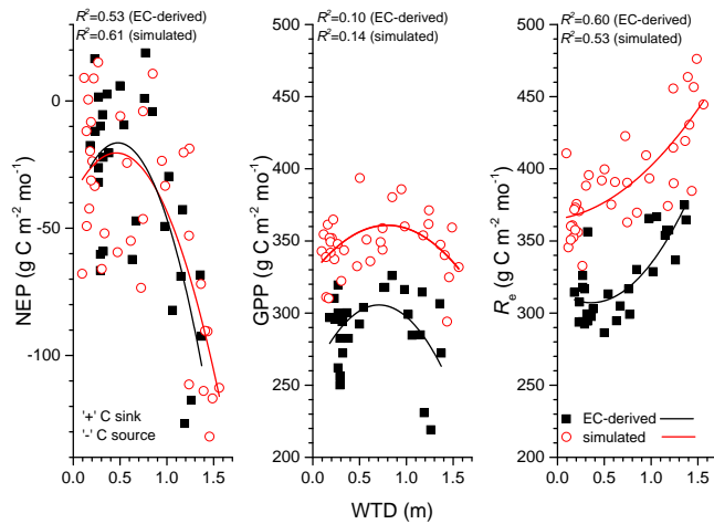
Fig. 8. Relationships between monthly simulated net ecosystem productivity (NEP), gross primary productivity (GPP) and ecosystem respiration ( R_e ), and monthly averaged simulated water table depths (WTD) (from Figs. 2c, 3c and 4c for 2002, 2003 and 2004 respectively); and monthly EC-derived NEP (derived from EC-gap filled hourly CO 2 fluxes), GPP and R_e (calculated from monthly averaged daily values digitally obtained from Hirano et al., 2007), and monthly averaged observed WTDs (from Figs. 2c, 3c and 4c for 2002, 2003 and 2004 respectively) during 2002–2004 over a drainage affected tropical peat swamp forest at Palangkaraya, Indonesia.
