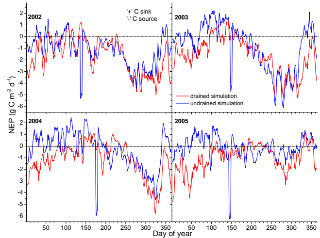
Fig. 10. Five-day moving averages of simulated daily net ecosystem productivity (NEP) for drained vs. undrained simulations (Sect. 2.2.6) during 2002–2005 over a drainage affected tropical peat swamp forest at Palangkaraya, Indonesia. Drained values are the same as those in Figs. 2–5.
