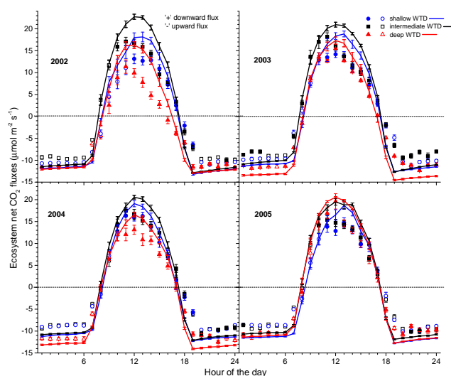
Fig. 7. Hourly binned simulated (lines) and EC-gap filled (symbols) ecosystem net CO 2 fluxes during shallow (DOY 1–30, 41–70, 11–40 and 41–70 in 2002, 2003, 2004 and 2005 respectively), intermediate (DOY 121–150, 146–175, 181–210 and 121–150 in 2002, 2003, 2004 and 2005 respectively) and deep (DOY 251–280, 251–280, 291–320 and 241–270 in 2002, 2003, 2004 and 2005 respectively) water table depth (WTD) hydroperiods (delineated by vertical dotted lines in Figs. 2–5) over a drainage affected tropical peat swamp forest at Palangkaraya, Indonesia. Solid symbols are averages of 30 hourly values more than 1/3 of which were EC measured CO 2 fluxes recorded at u^* > 0.17 \text{ m s}^{-1} . Open symbols are averages of 30 hourly values less than 1/3 of which were EC measured CO 2 fluxes recorded at u^* > 0.17 \text{ m s}^{-1} . Bars represent standard errors of means.
