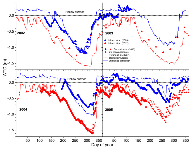
Fig. 9. Simulated daily drained vs. undrained water table depths (WTD) (Sect. 2.2.6) during 2002–2005 over a drainage affected tropical peat swamp forest at Palangkaraya, Indonesia. Drained WTDs are the same as those in Figs. 2c, 3c, 4c and 5c for 2002, 2003, 2004 and 2005 respectively. Negative values of WTD mean depths below the hollow surface and positive values mean depths above the hollow surface.
