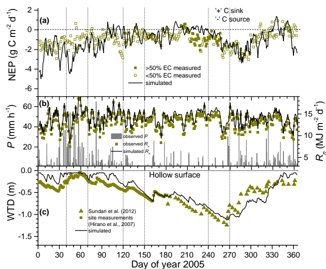
Fig. 5. (a) Three day moving averages of simulated and EC-gap filled estimates of net ecosystem productivity (NEP). Solid squares indicate sums of 24 values more than 1/2 of which were recorded at u^* (friction velocity) > 0.17 \text{ m s}^{-1} and open squares indicate sums of 24 values more than 1/2 of which were gap-filled; (b) hourly measured precipitation ( P ) and three day moving averages of simulated and measured net radiation ( R_n ); and (c) daily measured (values digitally obtained from Sundari et al., 2012 and measured in situ as mentioned in Hirano et al., 2007) and modelled water table depths (WTD) from hollow surface during 2005 over a drainage affected tropical peat swamp forest at Palangkaraya, Indonesia. Negative values of WTD mean depths below the ground.
