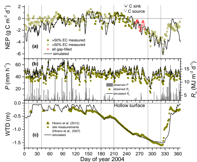
Fig. 4. (a) Three day moving averages of simulated and EC-gap filled estimates of net ecosystem productivity (NEP). Solid squares indicate sums of 24 values more than 1/2 of which were recorded at u^* (friction velocity) > 0.17 \text{ m s}^{-1} , open squares indicate sums of 24 values more than 1/2 of which were gap-filled, and open triangles indicate sums of 24 values all of which were gap-filled; (b) hourly measured precipitation ( P ) and three day moving averages of simulated and measured net radiation ( R_n ); and (c) monthly measured (values digitally obtained from Hirano et al., 2012), daily measured (site measurements mentioned in Hirano et al., 2007) and daily modelled water table depths (WTD) from hollow surface during 2004 over a drainage affected tropical peat swamp forest at Palangkaraya, Indonesia. Negative values of WTD mean depths below the ground.
