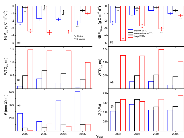
Fig. 6. (a) Average simulated daily net ecosystem productivity (NEP sim ) (b) average EC-gap filled daily net ecosystem productivity (NEP EC-gap ) (c) average simulated water table depths (WTD sim ) (d) average observed water table depths (WTD obs ) (e) total observed precipitation ( P ), and (f) average mid-day (10:00–14:00 LT) vapour pressure deficit ( D ) during shallow (DOY 1–30, 41–70, 11–40 and 41–70 in 2002, 2003, 2004 and 2005 respectively), intermediate (DOY 121–150, 146–175, 181–210 and 121–150 in 2002, 2003, 2004 and 2005 respectively) and deep (DOY 251–280, 251–280, 291–320 and 241–270 in 2002, 2003, 2004 and 2005 respectively) water table depth (WTD) hydroperiods (delineated by vertical dotted lines in Figs. 2–5) over a drainage affected tropical peat swamp forest at Palangkaraya, Indonesia. Bars represent standard errors of means. Asterisks (**) at the top of a column represent significant ( P < 0.01 ) difference from the adjacent column(s).
