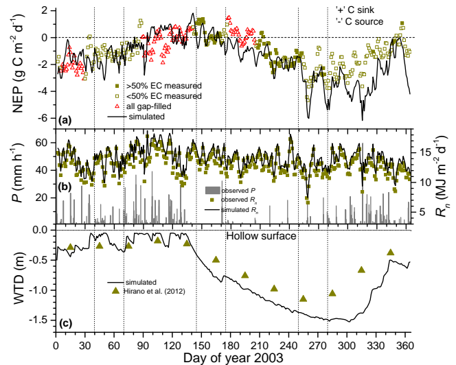
Fig. 3. (a) Three day moving averages of simulated and EC-gap filled estimates of net ecosystem productivity (NEP). Solid squares indicate sums of 24 values more than 1/2 of which were recorded at u^* (friction velocity) > 0.17 \text{ m s}^{-1} , open squares indicate sums of 24 values more than 1/2 of which were gap-filled, and open triangles indicate sums of 24 values all of which were gap-filled; (b) hourly measured precipitation ( P ) and three day moving averages of simulated and measured net radiation ( R_n ); and (c) monthly measured (values digitally obtained from Hirano et al., 2012) and daily modelled water table depths (WTD) from hollow surface during 2003 over a drainage affected tropical peat swamp forest at Palangkaraya, Indonesia. Negative values of WTD mean depths below the ground.
