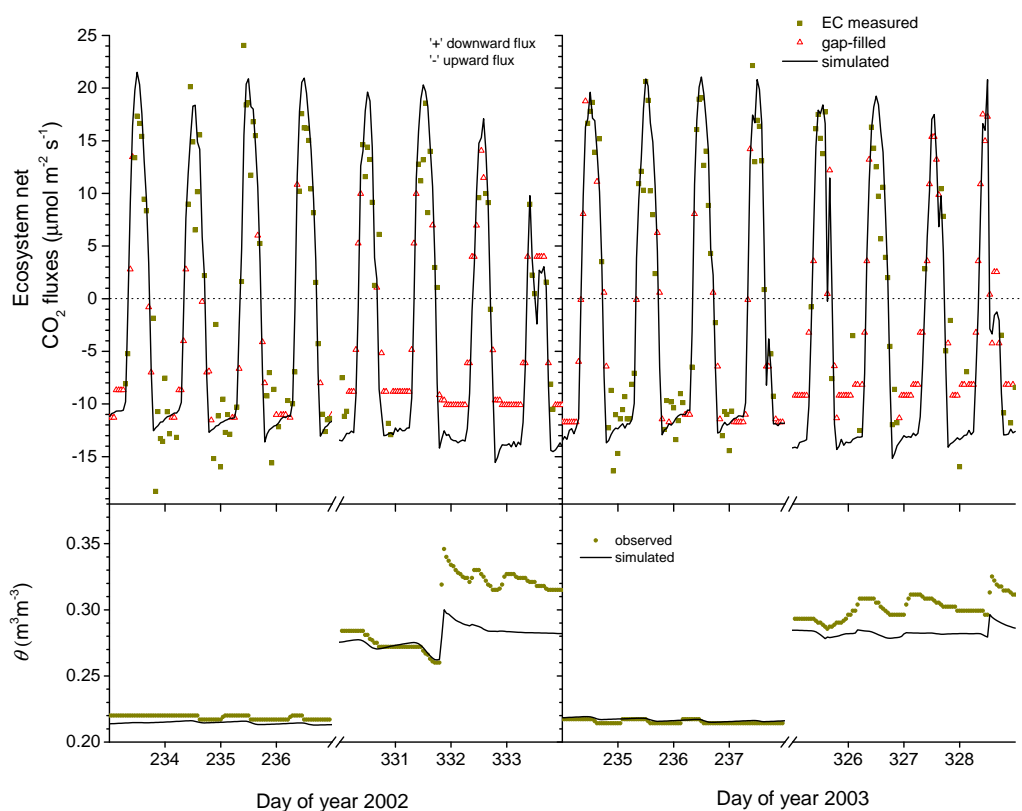
Fig. 1. Hourly EC measured, gap-filled and simulated net ecosystem CO 2 fluxes and observed and simulated soil water contents ( \theta ) from 0–0.20 m depth of the hummock during 2002 and 2003 over a drainage affected tropical peat swamp forest at Palangkaraya, Indonesia.
