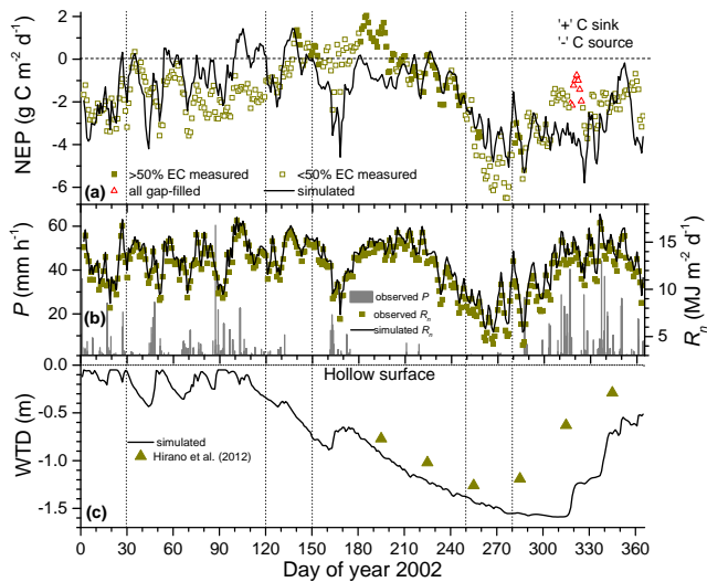
Fig. 2. (a) Three day moving averages of simulated and EC-gap filled estimates of net ecosystem productivity (NEP). Solid squares indicate sums of 24 values more than 1/2 of which were recorded at u^* (friction velocity) > 0.17 \text{ m s}^{-1} , open squares indicate sums of 24 values more than 1/2 of which were gap-filled, and open triangles indicate sums of 24 values all of which were gap-filled; (b) hourly measured precipitation ( P ) and three day moving averages of simulated and measured net radiation ( R_n ); and (c) monthly measured (values digitally obtained from Hirano et al., 2012) and daily modelled water table depths (WTD) from hollow surface during 2002 over a drainage affected tropical peat swamp forest at Palangkaraya, Indonesia. Negative values of WTD mean depths below the ground.
