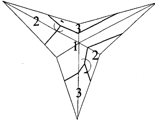
Figure 5.5: A perturbation of an index -2 component
