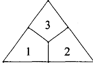
Figure 3.3: The canonical division \Delta_*^{m-1}
