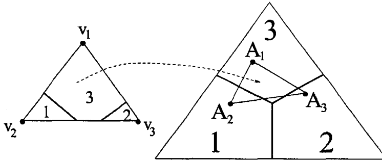
Figure 3.12: The mapping f_v
