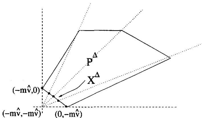
Figure 2.3: The simplicial division of X^\Delta
