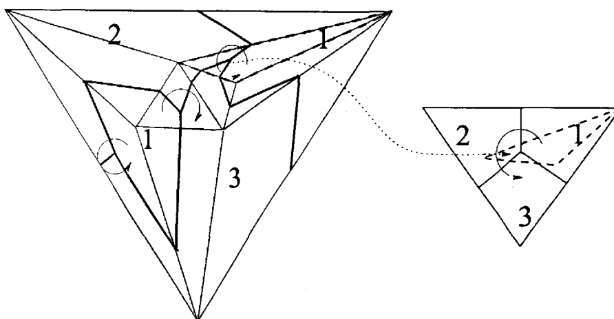
Figure 3.15: The orientation of the X^\Delta and \Delta^{m-1}
