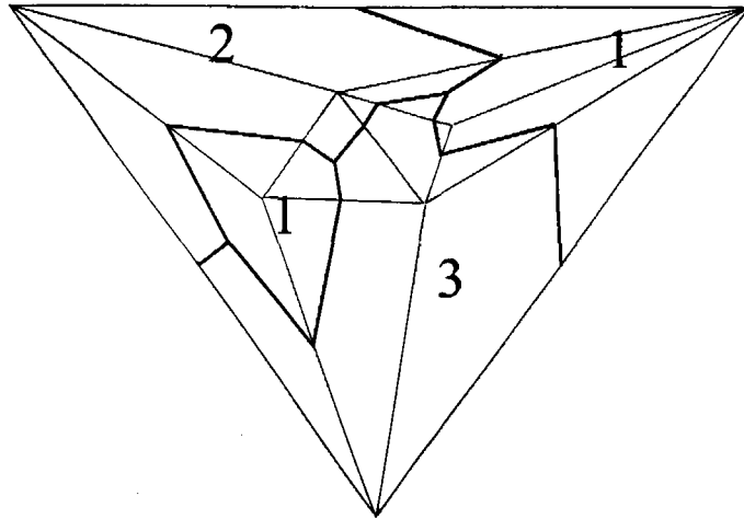
Figure 2.6: The labelled dual construction X_*^\Delta for Example 2.3
