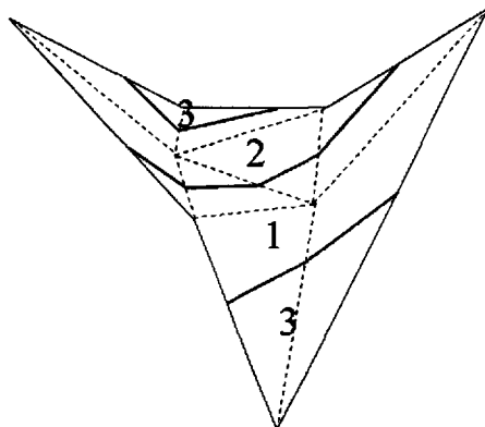
Figure 6.10: An approximation of the homotopy
