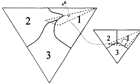
Figure 4.7: A homotopy
