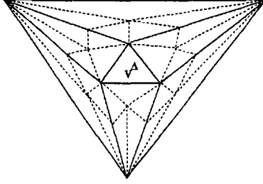
Figure 4.5: The regular refinement obtained from the iterated pseudo refinement
