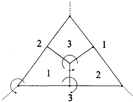
Figure 1.6: The index in the coordination game
