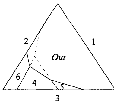
Figure 1.9: The division of X for the game G^2 with outside option
