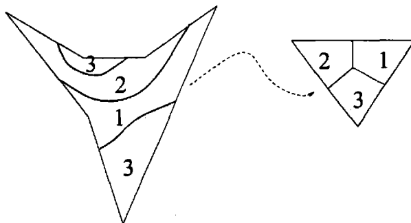
Figure 6.9: A homotopy for outside option equilibrium components
