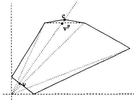
Figure 3.9: An iterated refinement of |X^\Delta|
