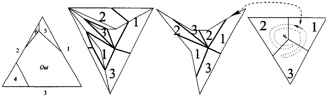
Figure 6.5: An index zero essential component
