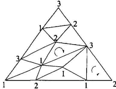
Figure 3.1: A labelled triangulation
