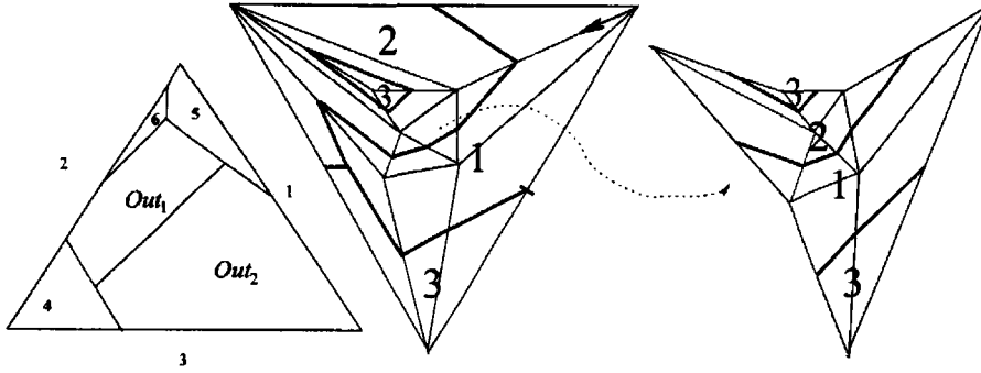
Figure 6.8: Duplication of the outside option
