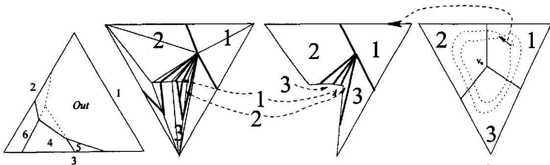
Figure 5.4: An outside option component with index +2
