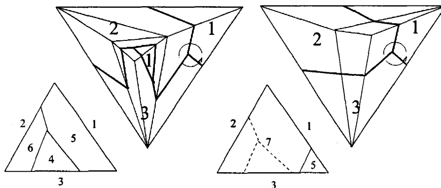
Figure 4.1: An index +1 equilibrium in H^-
