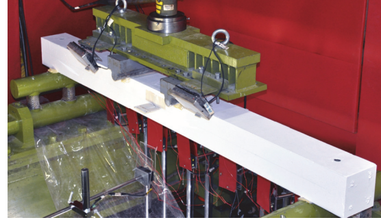
Photo 2: Experimental setup
