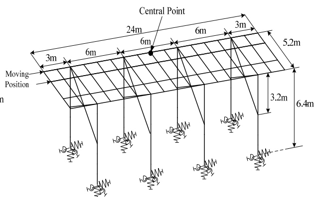
Figure 5: Reinforcement model 2
