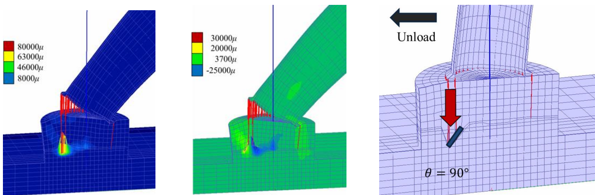
(a) Principal strain contour (b) Shear strain contour (c) Magnified deformation (disp. x50)
