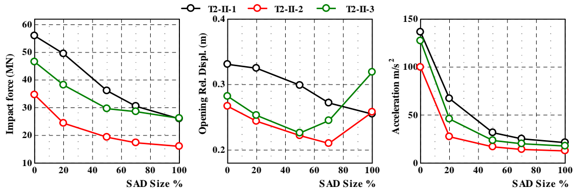
Figure 8 Peak responses variation with SAD size
