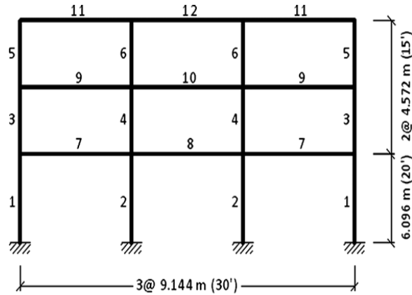
Figure 3: The first structure model (Safari, 2011).
