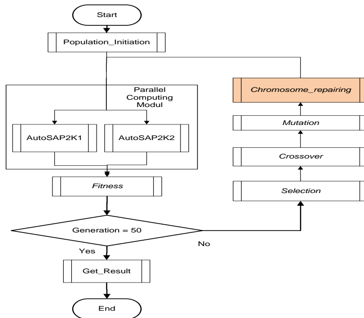
Figure 2: Flowchart of GACR-SAP2000.
