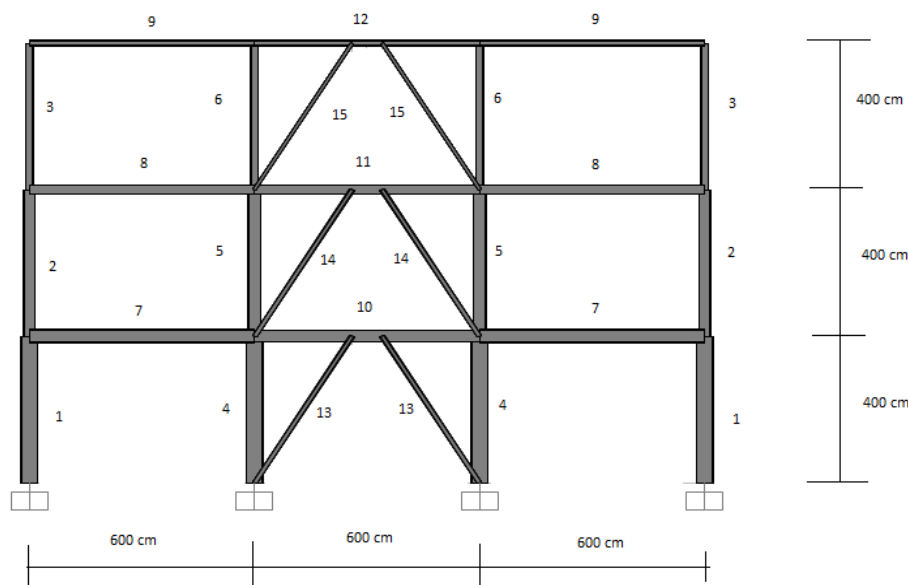
Figure 4: The second structure model (Joni, 2012).
