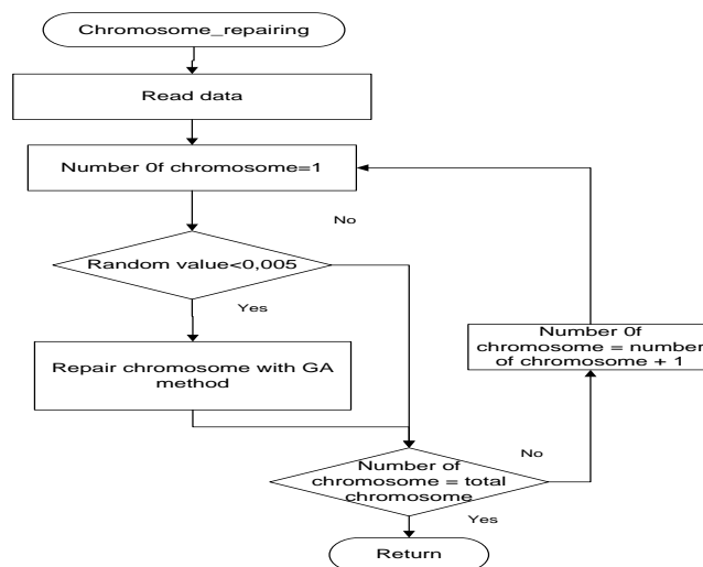
Figure 1: Flowchart of chromosome repairing.
