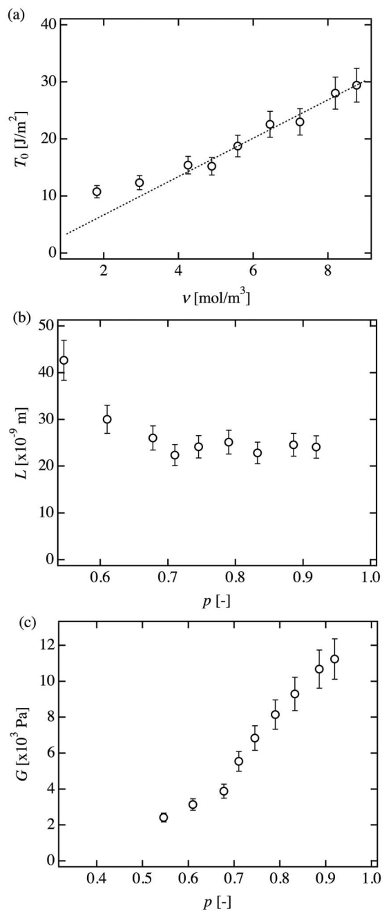
FIG. 2. (a) Fracture energy ( T_0 ) as a function of v . The dotted line is the linear fitting showing the relationship, T_0 \sim v . (b) L as a function of p . (c) G as a function of p for p -tuned Tetra-PEG gel.
