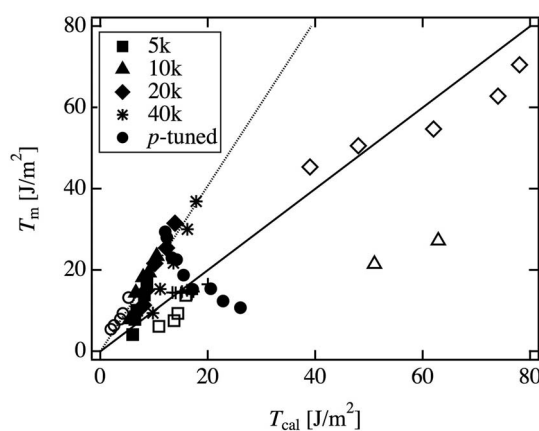
FIG. 6. The fracture energy measured ( T_m ) and calculated ( T_{cal} ) for Tetra-PEG gels with different p , N , and \phi_0 . The values of T_m and T_{cal} of different gels and elastomers are taken from the literatures: cis-polyisoprene, unfilled triangles; 4 poly(dimethylsiloxane), unfilled rhombuses; 4 swollen poly(dimethylsiloxane), crosses; 4 polyacrylamide hydrogels, unfilled circles; 31 and squares. 32 The solid line shows the relationship T_m = T_{cal} , and dotted line shows the guide of the linear relationship between T_m and T_{cal} of Tetra-PEG gels.
