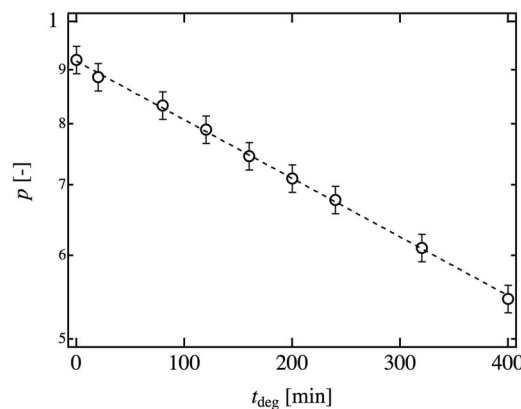
FIG. 1. Reaction conversion ( p ) as a function of t_{\text{deg}} . The dashed line is the guide line showing the relationship, p \sim \exp(-t_{\text{deg}}) .
