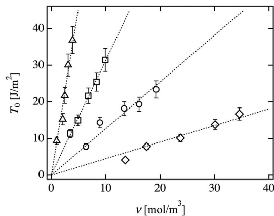
FIG. 3. T_0 as a function of v in the Tetra-PEG gels (5k, rhombus; 10k, circle; 20k, square; 40k, triangle). Linear fitting of the data are shown as the dotted lines.
