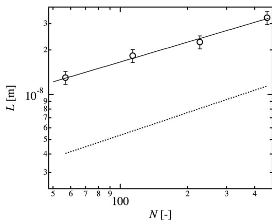
FIG. 4. L as a function of N in Tetra-PEG gel. The solid line is the fitting line of a power function ( L \sim N^{0.45} ), and the dashed line is the guide showing the computed R_0 of network chain with polymerization degree of N .
