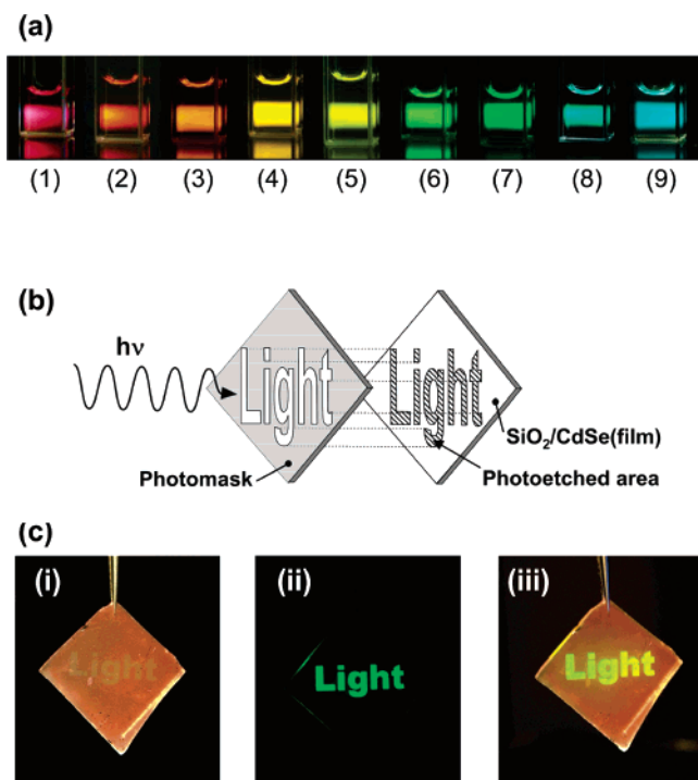
Figure 3. (a) Photographs of UV-illuminated \text{SiO}_2/\text{CdSe} (col) solutions photoetched at 630 (1), 620 (2), 610 (3), 600 (4), 590 (5), 575 (6), 560 (7), 532 (8), and 514 nm (9). The excitation wavelength was 350 nm. (b) Schematic illustration of the patterned monochromatic irradiation on \text{SiO}_2/\text{CdSe} (film). (c) Photographs of photoetched \text{SiO}_2/\text{CdSe} (film) placed under room light (i), ultraviolet light (350 nm) (ii), and both lights (iii). Original CdSe particles were prepared at (a) 175 and (c) 150 °C.
