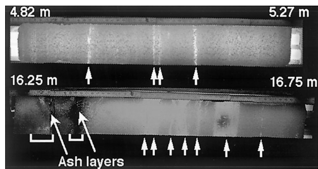
Fig. 5. Ice-core sections showing two representative layers: firn layers that have not been affected by melting (whitish parts) and melt features formed by melting and subsequent freezing (clear parts indicated by arrows). Two layers of melt features associated with ash layers are found at the top of the lower core section.
