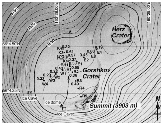
Fig. 2. A plan view of the summit craters, Gorshkov and Herz, and the distribution of annual mass balance (m) for 1997/98. Arrows denote a principal flow direction indicated by the surface gradient. Subsurface caves starting from an ice cave at the southwest rim are clearly indicated by depressions along the west to northwestern rim of the Gorshkov crater.
