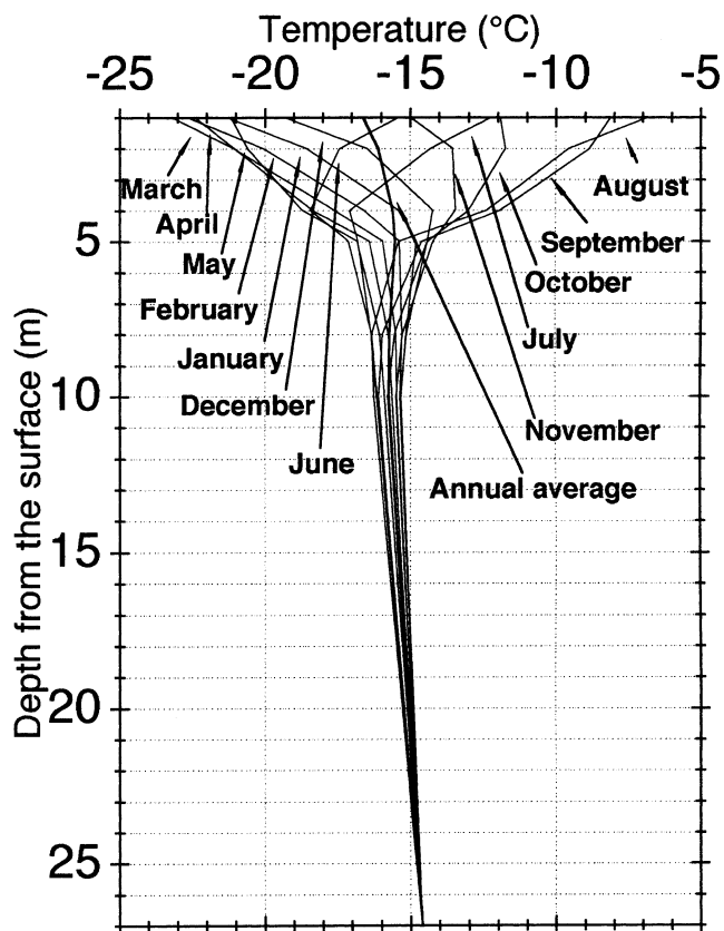
Fig. 4. Monthly and annual average snow-temperature profiles measured at BHI (Gorshkov crater) from August 1996 to July 1997.
