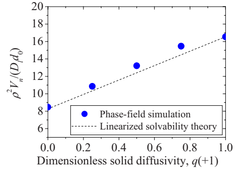
FIG. 7. (Color online) Comparison of dependence of \rho^2 V_n on q(+1) between the present model (solid circle) and the linearized solvability theory (dashed line). The calculations were performed with \Omega = 0.55 , \varepsilon_4 = 0.02 , k = 1.0 , and d_0/W_0 = 0.277 .
