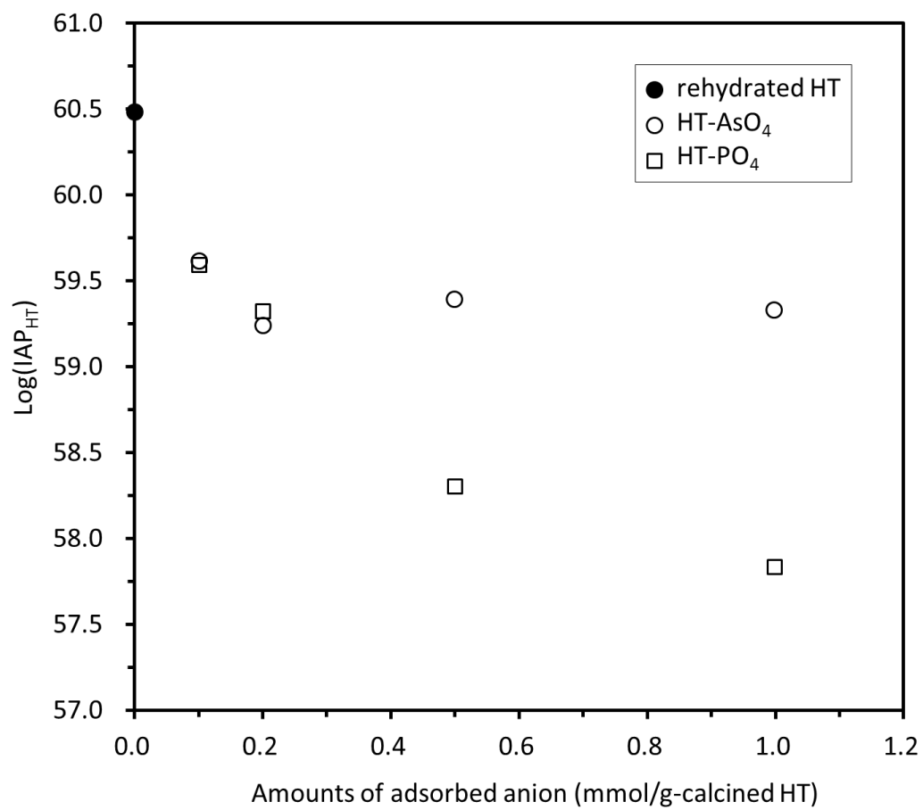
Fig. 6. IAP_{HT} in the reacted solutions as a function of the amount of adsorbed anions.
