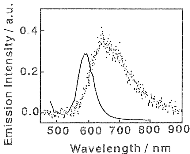
Figure 1.5.5. ECL spectrum of the \text{Ru}(\text{bpy})_3^{2+}(\text{C}_{11}\text{SH})_2 SAM modified ITO electrode in a solution containing 0.4 M \text{Na}_2\text{SO}_4 and 0.1 M \text{Na}_2\text{C}_2\text{O}_4 at +1150 mV (dots) and the emission spectrum of \text{Ru}(\text{bpy})_3^{2+}(\text{C}_{11}\text{SH})_2 in \text{CH}_2\text{Cl}_2 solution (solid line).
