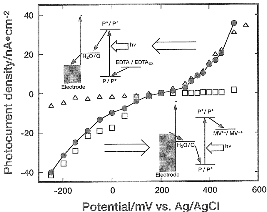
Figure 1.5.6. Potential dependence of the photocurrent at the gold electrode modified with the PQSH SAM. Solutions contain 0.1 M \text{Na}_2\text{SO}_4 (pH = 4.5) and (a) 50 mM EDTA and 5 mM \text{MV}^{2+} (closed circle), (b) 50 mM EDTA (open triangle) and (c) 5 mM \text{MV}^{2+} (open square). The insets illustrate the energy diagram of the electrode/electrolyte interface when the electrode potential was more positive (upper) or more negative (lower) than the redox potential of quinone moiety.
