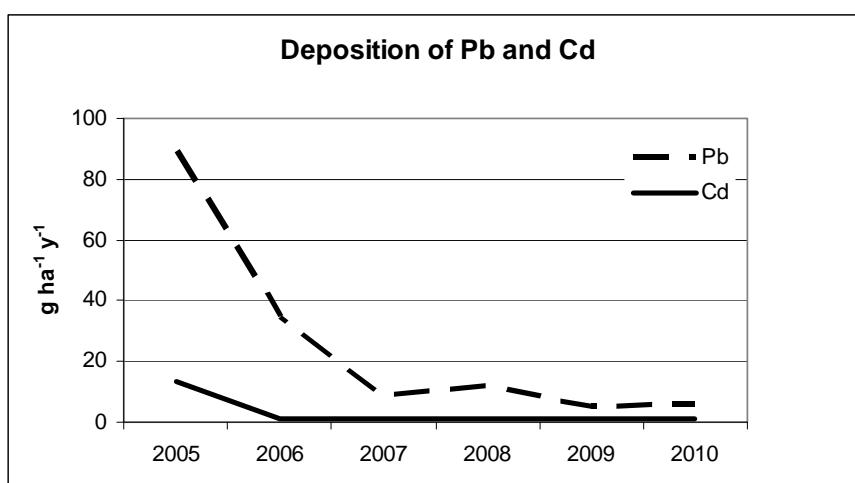
Fig. 2. Mean annual deposition of Pb and Cd during the period 2005-2010 at the Petrohan site, g ha -1 yr -1 .
