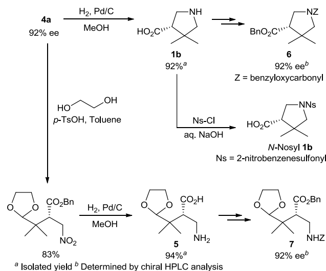
Scheme 1 Transformation of 4a to a cyclic γ-amino acid 1b and a linear β-amino acid 5
