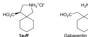
Fig. 1 Gabapentin and its analogue
