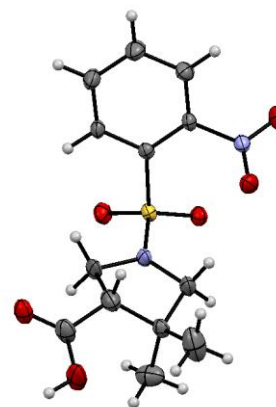
Scheme 1 Transformation of 4a to a cyclic γ-amino acid 1b and a linear β-amino acid 5
