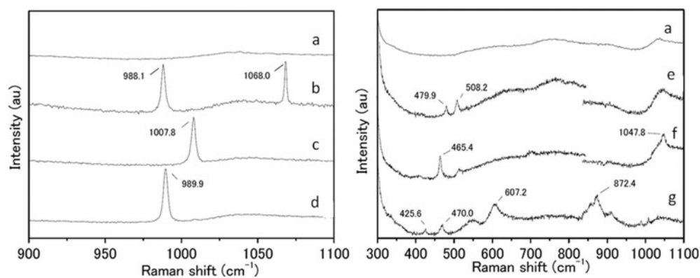
Fig. 2. Typical Raman spectra of microparticles found during Termination I in the Dome Fuji ice core: (a) ice, (b) mixture of sulfate and nitrate salts, (c) \text{CaSO}_4 \cdot 2\text{H}_2\text{O} (gypsum), (d) \text{Na}_2\text{SO}_4 \cdot 10\text{H}_2\text{O} (mirabilite) or \text{MgSO}_4 \cdot 11\text{H}_2\text{O} (meridianiite), (e) feldspar, (f) \text{SiO}_2 (quartz) and (g) an unknown spectrum.
