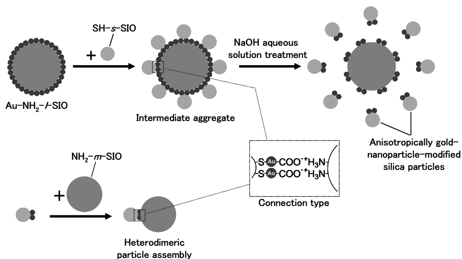
Scheme 1 Diagram of method for preparing heterodimeric particle assemblies.
