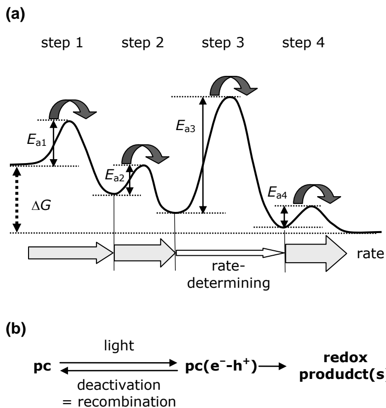
Fig. 9 (a) Model interpreting a rate-determining step in a 4-step series reaction. Step 3 with largest activation energy determines the overall rate. (b) Simplified scheme of photocatalytic reaction with a photocatalyst "pc". It is clear that this process is not a series reaction since a "deactivation step" is included.
