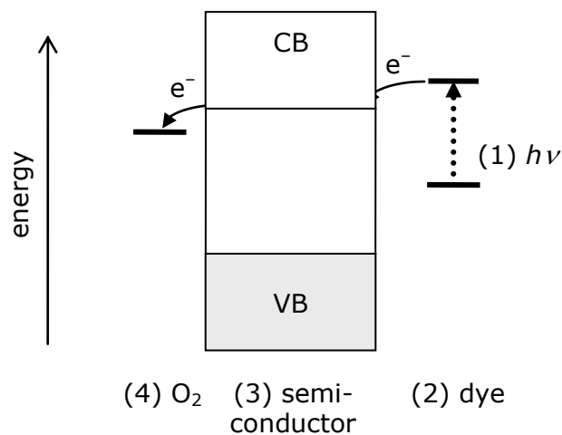
Fig. 11 Possible mechanism of "dye-sensitized" photoinduced oxidative decomposition of dye in the presence of oxygen. Components (1)–(4) are necessary conditions for "dye-sensitized reaction" and they are also necessary conditions for ordinary photocatalytic reaction.
