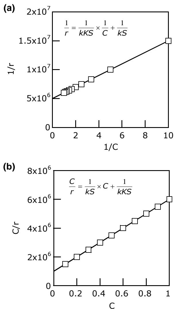
Fig. 7 Simulation of linearized plots for kinetics governed by surface concentration of substrates adsorbed on the photocatalyst surface in a Langmuirian fashion, where r , C , k , K and S are rate of reaction ( \text{mol s}^{-1} ), concentration of a substrate ( \text{mol L}^{-1} ), rate constant ( 10^{-4} \text{ s}^{-1} ), adsorption equilibrium constant ( 5 \text{ L mol}^{-1} ) and saturated amount of adsorption ( 2 \times 10^{-3} \text{ mol} ).
