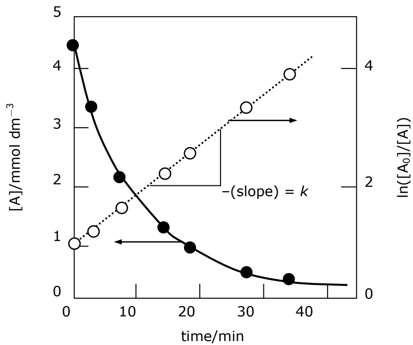
Fig. 6 First-order kinetic analysis for a reaction consuming a substrate A. Plot of logarithm of relative consumption (in the present plot, ratio of initial concentration of substrate A and concentration of A at a given time).
