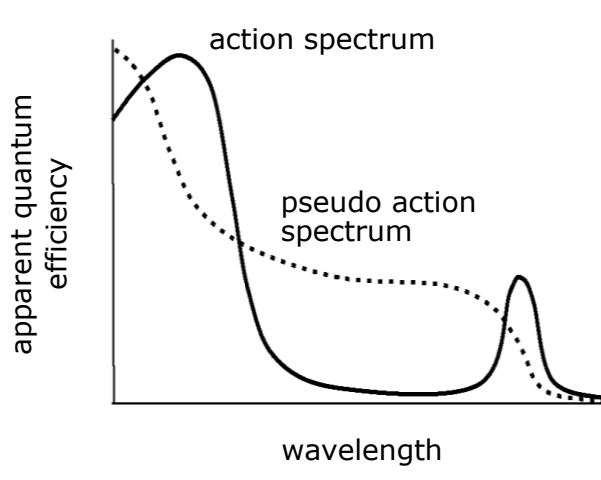
Fig. 12 Examples of action and pseudo action spectra for photoinduced reaction by an ordinary semiconductor photocatalyst (shorter wavelength) and an organic dye (longer wavelength peak). A pseudo action spectrum taken by cut-off filters corresponds to integration of the "true" action spectrum from the longer-wavelength side.
