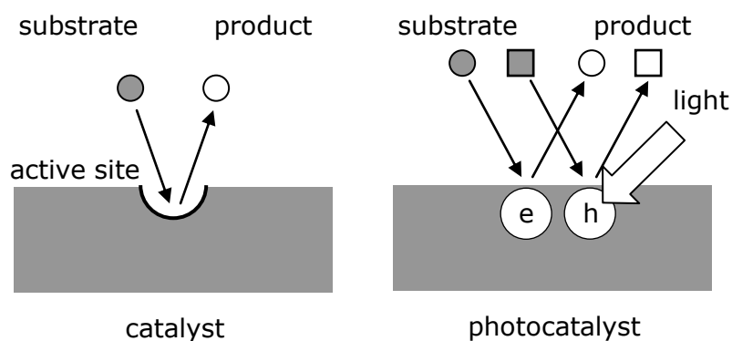
Fig. 1 Difference in concepts of catalytic and photocatalytic reactions: A catalyst contains active sites at which a substrate is converted into a product, while no active sites are present on a photocatalyst.
