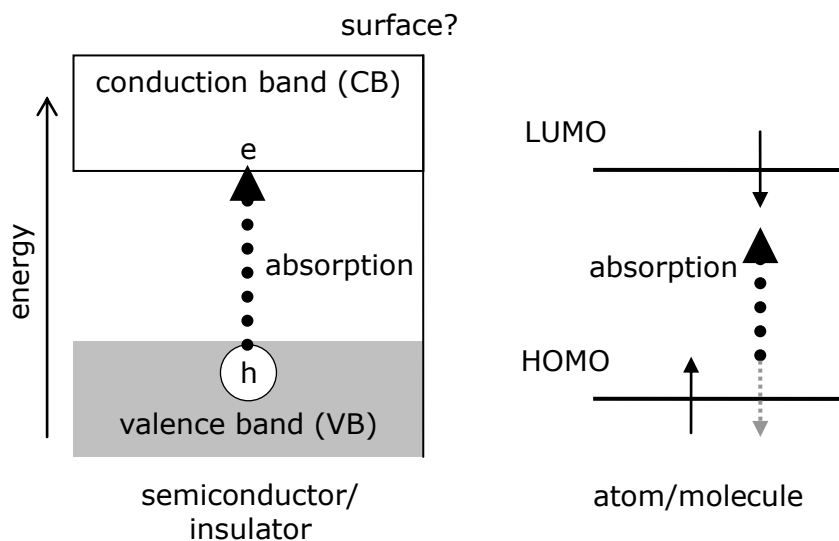
Fig. 3 Photoabsorption by transition of electrons in the VB or HOMO to the CB or LUMO in a semiconductor/insulator or atom/molecule, respectively.
