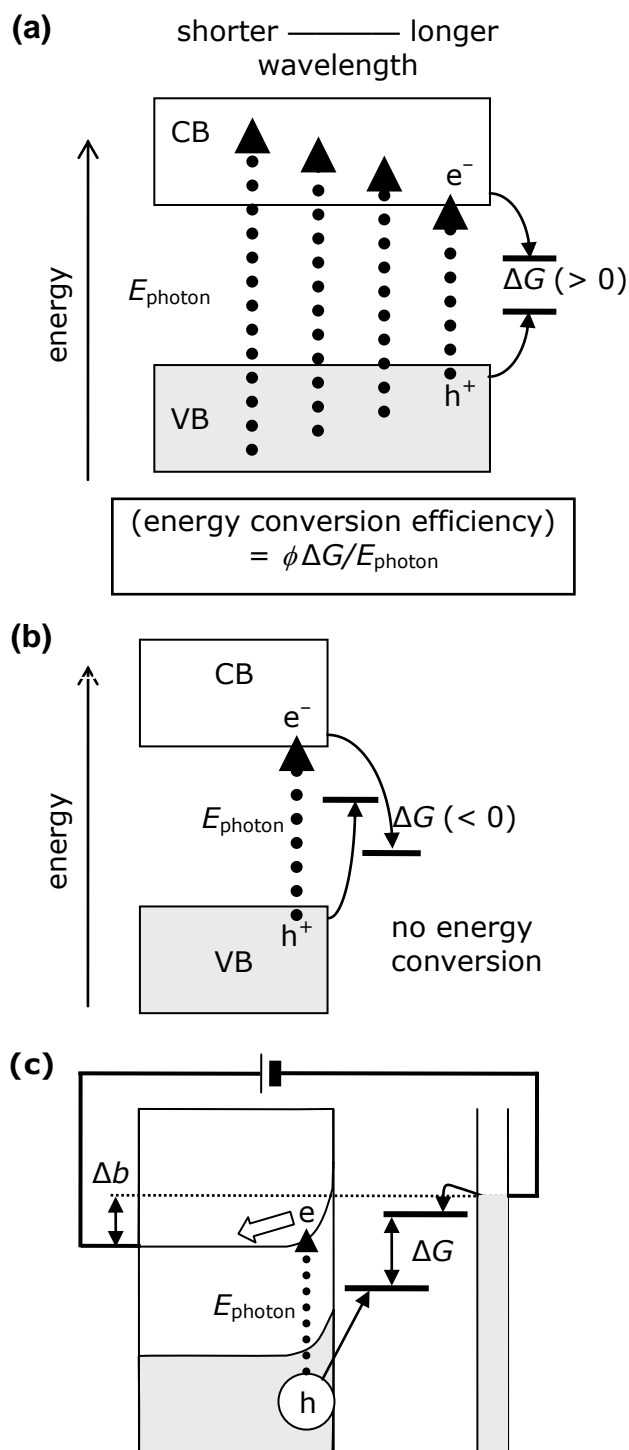
Fig. 5 (a) Photo-to-chemical energy conversion efficiency of photocatalytic reaction calculated as an integral of the product of apparent quantum efficiency ( \phi ) and Gibbs energy change (storage) divided by photon energy ( E_{\text{photon}} ) as a function of wavelength. (b) In the case where Gibbs energy change is negative, energy conversion efficiency can not be defined, or is defined to be zero. (c) Electrochemically biased ( \Delta b ) photoelectrochemical cell consisting of an n-type semiconductor and metal counter electrodes.
