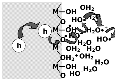
Fig. 4 Transfer of positive holes from bulk of a photocatalyst through the interface to aqueous solution phase. Surface-adsorbed and free (hydrated) hydroxyl radicals and its derivatives can be a possible form of positive holes.
