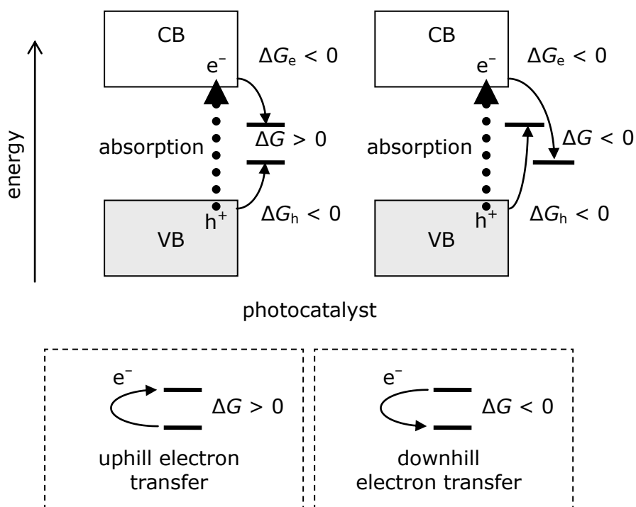
Fig. 2 Gibbs-energy change in photocatalytic reactions.
