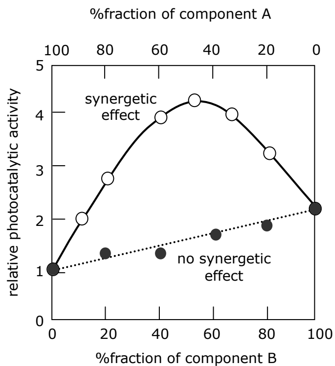
Fig. 14 Hypothetical representation of relative photocatalytic activities of mixtures of components A and B. A synergetic effect can be suggested at least when a mixture shows better photocatalytic activity compared with those of pure components A and B.
