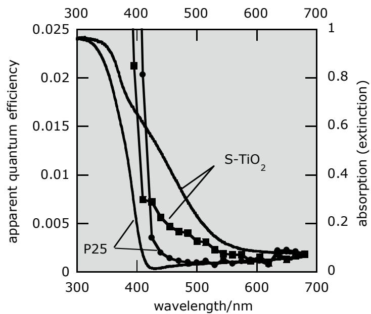
Fig. 10 Diffuse reflectance (photoabsorption) and action spectra for acetic acid, having no absorption in the visible-light wavelength range, decomposition in aerated aqueous solutions of sulfur-doped titania (S-TiO 2 ) and Degussa (Evonic) P25.
