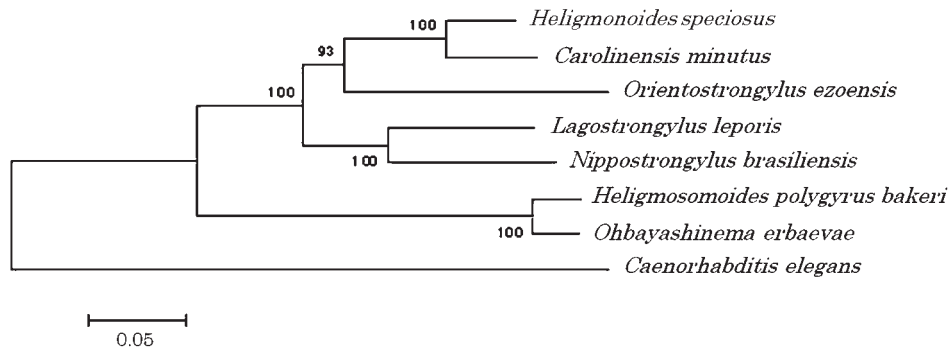
Fig. 1A. Phylogenetic relationships in the ITS-1 sequences of the five species of Heligmonellidae nematodes by the neighbor-joining method. Values on the tree nodes are bootstrap proportions (%). The scale bar represents divergence of 0.05.
