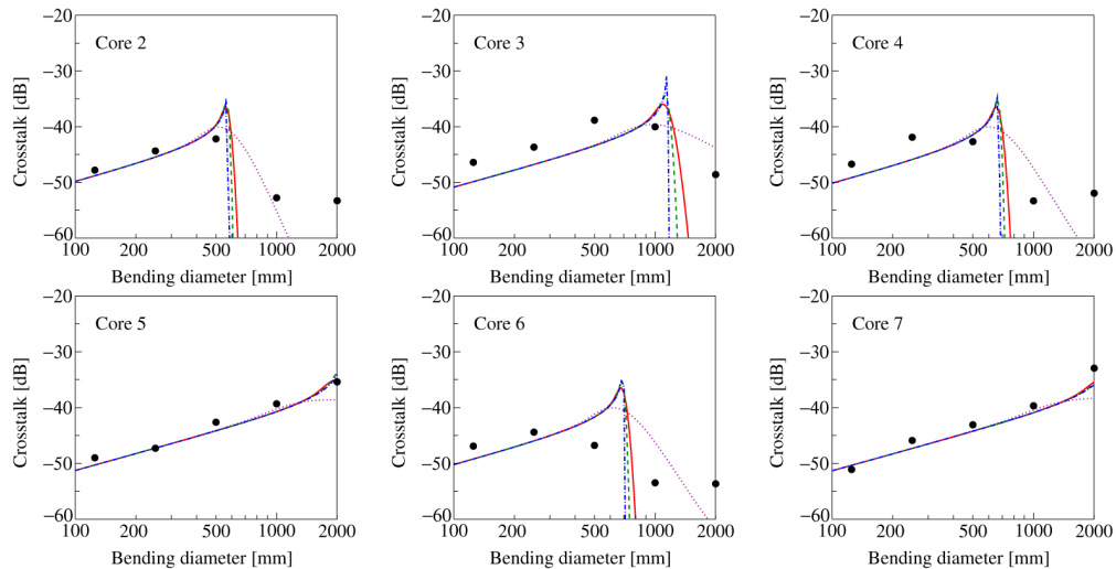
Fig. 8. Bending-diameter dependence of crosstalk calculated from coupled-power theory with Gaussian autocorrelation function. Dotted line: d_c = 0.01 m, solid line: d_c = 0.05 m, dashed line: d_c = 0.1 m, dashed and dotted line: d_c = 0.5 m, closed circles: measured data [4].
