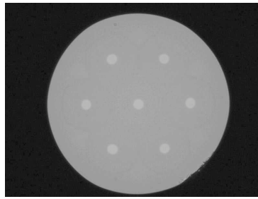
Fig. 3. Cross-section of a quasi-homogeneous 7-core fiber [4].
