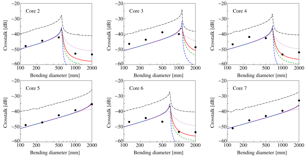
Fig. 5. Bending-diameter dependence of crosstalk calculated from coupled-power theory with exponential autocorrelation function. Dotted line: d_c = 0.01 m, solid line: d_c = 0.05 m, dashed line: d_c = 0.1 m, dashed and dotted line: d_c = 0.5 m, dashed and double-dotted line: Eq. (25) [4], closed circles: measured data [4].
