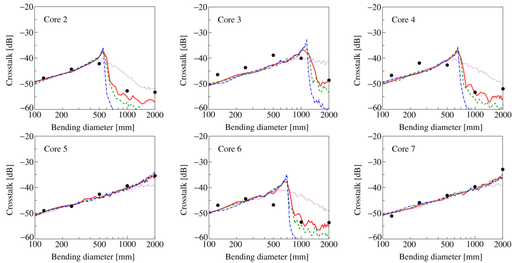
Fig. 4. Bending-diameter dependence of crosstalk calculated from coupled-mode theory. Dotted line: d_s = 0.01 \text{ m} , solid line: d_s = 0.05 \text{ m} , dashed line: d_s = 0.1 \text{ m} , dashed and dotted line: d_s = 0.5 \text{ m} , closed circles: measured data [4].
