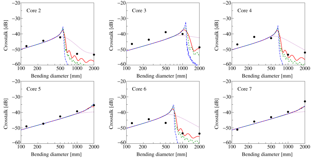
Fig. 9. Bending-diameter dependence of crosstalk calculated from coupled-power theory with triangular autocorrelation function. Dotted line: d_c = 0.01 m, solid line: d_c = 0.05 m, dashed line: d_c = 0.1 m, dashed and dotted line: d_c = 0.5 m, closed circles: measured data [4].
