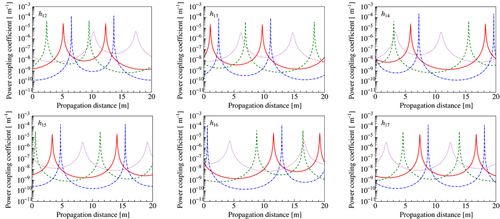
Fig. 6. Propagation-distance dependence of power-coupling coefficients for bending diameter of 250 mm. Dotted line: d_c = 0.01 m, solid line: d_c = 0.05 m, dashed line: d_c = 0.1 m, dashed and dotted line: d_c = 0.5 m.
