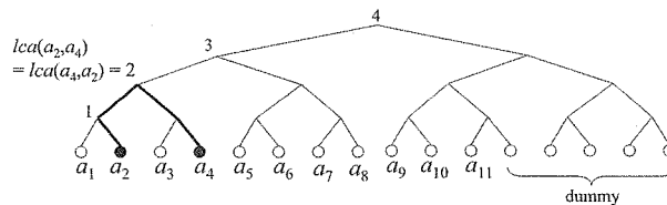
Fig. 2 The alphabet tree for \Sigma \cup \hat{N} = \{a_1, \dots, a_{11}\} .
