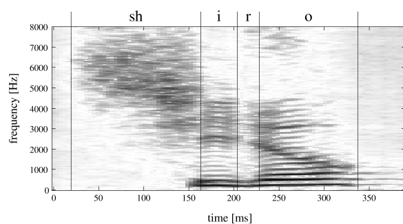
Fig. 3 Spectrogram of the original speech data “shiro”.
