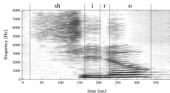
Fig. 5 Spectrogram of the band-extended speech data “shiro” with the proposed technique.
