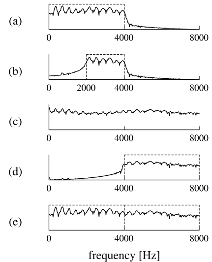
Fig. 1 Procedure of the band extension technique based on full wave rectification: (a) original speech, (b) band-pass filtering, (c) full wave rectification, (d) high-pass filtering, and (e) mixing the low and high bands.
