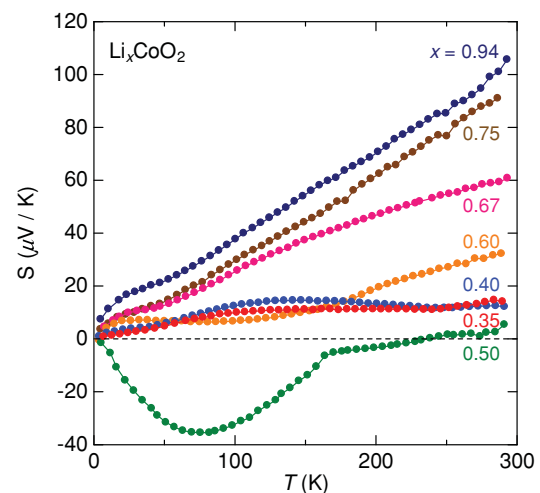
FIG. 5. (Color online) Temperature dependence of Seebeck coefficient ( S ) for the x = 0.35, 0.40, 0.50, 0.60, 0.67, 0.75, and 0.94 samples.
