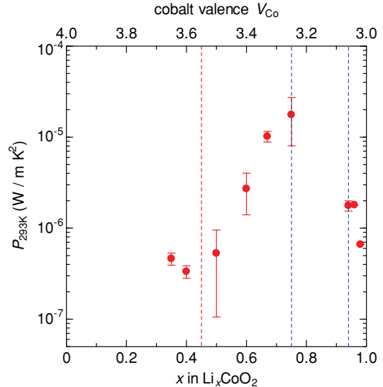
FIG. 7. (Color online) The thermoelectric power factor P \equiv S^2/\rho for the \text{Li}_x\text{CoO}_2 samples. The P values were calculated from the \rho and S values at 293 K.
