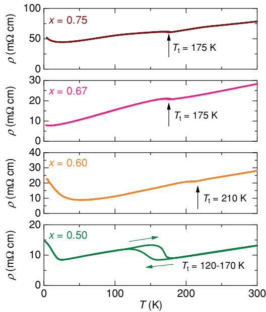
FIG. 2. (Color online) Temperature dependence of electrical resistivity ( \rho ) for the x = 0.50, 0.60, 0.67, and 0.75 samples.
