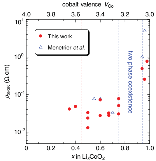
FIG. 4. (Color online) The magnitude of electrical resistivity at 293 K ( \rho_{293K} ) as a function of x in Li_xCoO_2 . For comparison, data plots of Ménétrier et al. (Ref. 27) are also shown with blue triangles.
