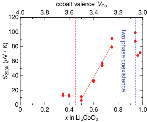
FIG. 6. (Color online) The magnitude of Seebeck coefficient at 293 K ( S_{293K} ) as a function of x in \text{Li}_x\text{CoO}_2 .
