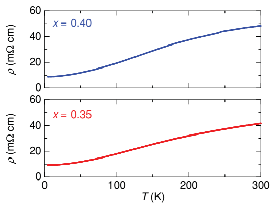
FIG. 3. (Color online) Temperature dependence of electrical resistivity ( \rho ) for the x = 0.35 and 0.40 samples.
