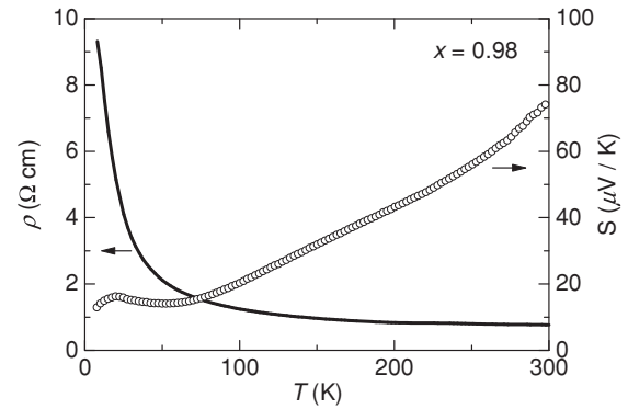
FIG. 8. Electrical resistivity ( \rho ) and Seebeck coefficient ( S ) of the x = 0.98 sample. These measurements were carried out simultaneously with a single piece of the bulk sample.
