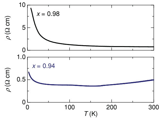
FIG. 1. (Color online) Temperature dependence of electrical resistivity ( \rho ) for the \text{Li}_x\text{CoO}_2 samples with x = 0.94 and 0.98.
