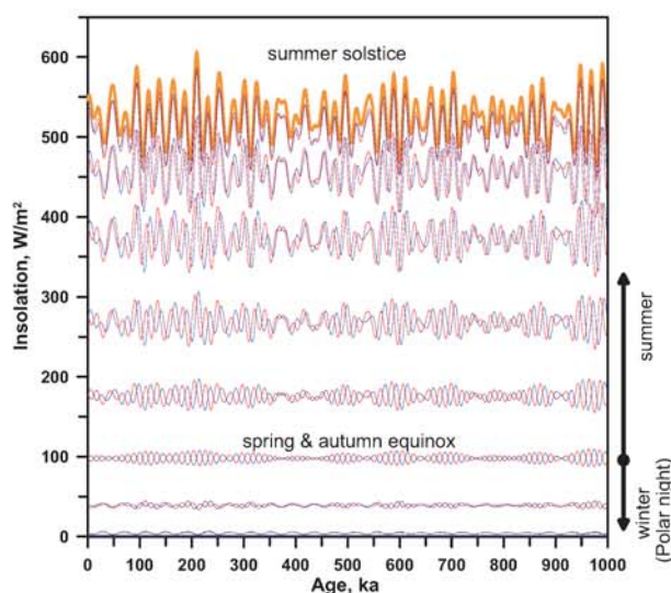
Figure 1: Calculated variations of the local daily average insolation at Dome Fuji over the past 1 Ma [11]. Each curve represents the variation of the local daily average insolation on a specific day of the year.
