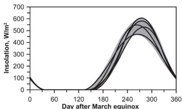
Figure 2: The full range of calculated local daily average insolation in the course of a year at Dome Fuji over the past 1Ma (grey area). Randomly chosen examples of five annual cycles are plotted in black to illustrate the variability in the width and height of the annual insolation cycles (calendar years have been transformed into standard years of 360 model days to be compatible with the model output. One model day corresponds to 1 degree change in the true longitude of the sun and thus 365.24/360 calendar days).
