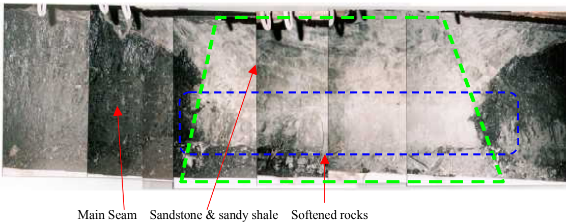
Fig. 7 Old roadway observed in Jobu Hidari No. 6 SD. Fragments of roof rock distributed in coal slurry (gray part seen around the top of the old roadway), the mixture of water and fine coal powder produced in coal processing.
