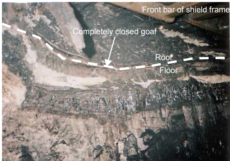
Fig. 15 A goaf of the Main seam mined in 1954, appeared at the working face of Jobu Hidari No.6 SD. The white broken line indicates the boundary between the roof and the floor of the excavated Main seam.
