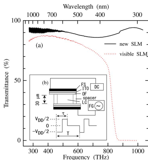
Fig. 1. (Color online) (a) Transmittance curves of UV-LC-SLM (solid curve) and visible LC-SLM (dotted curve). (b) Structure of UV-LC-SLM and applied voltage waveform. LC, liquid crystal; FS, fused silica substrate; ITO, indium tin oxide film; OF, oriented organic film; DC, DC power source; FG, function generator; T, period; \tau , pulse width.
