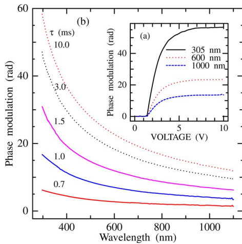
Fig. 3. (Color online) (a) Applied voltage dependence of phase modulation \Delta\phi at 305 (solid curve), 600 (dotted curve), and 1000 nm (dashed curve) under \tau=6.5 ms and T=13 ms. (b) Wavelength dependence of phase modulation for different widths ( \tau ) of applied voltage pulses at T=13 ms and V_{DD}=7.0 V.
