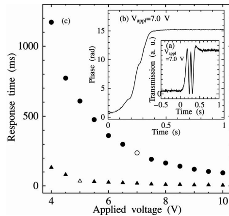
Fig. 4. Transient response of UV-LC-SLM at 633 nm. (a) Transmitted light intensity I(t) at V_{\text{appl}}=7.0 V. (b) Transient phase modulation calculated from I(t) at V_{\text{appl}}=7.0 V. (c) Applied voltage V_{\text{appl}} dependence of response time \tau_r for UV-LC-SLM (open circles, \tau_r at 7.0 V) and visible LC-SLM (open triangles, \tau_r at 5.0 V).
