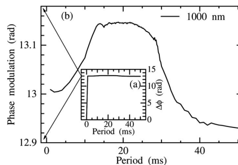
Fig. 2. (a) Period dependence of phase modulation \Delta\phi at 1000 nm, V_{\text{DD}}=6 V and \tau/T=0.5 . (b) Enlarged y axis.
