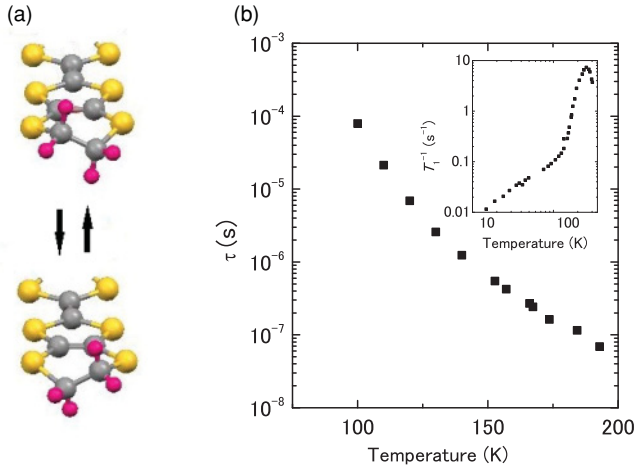
FIG. 3. (Color online) (a) Ethylene motion of the BEDT-TTF molecule. (b) Temperature dependence of \tau_c . Inset: temperature dependence of T_1^{-1} for \kappa -(BEDT-TTF) 2 Cu(NCS) 2 (data taken from Ref. 14).
