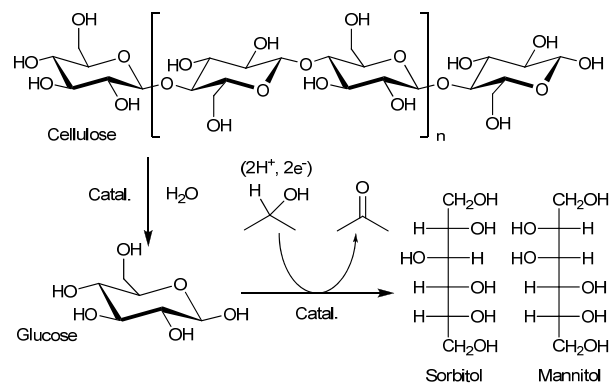
Scheme 1 Transfer hydrogenation of cellulose to sugar alcohols.
