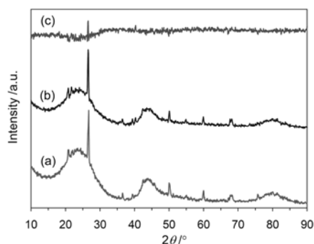
Fig. 1 XRD patterns of (a) AC(N), (b) Ru/AC(N) and (c) the differential pattern of (b)–(a).
