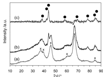
Fig. 2 XRD patterns of (a) Al 2 O 3 , (b) Ru/Al 2 O 3 and (c) the differential pattern of (b)–(a). Circles: Ru metal. x: \gamma -Al 2 O 3 .
