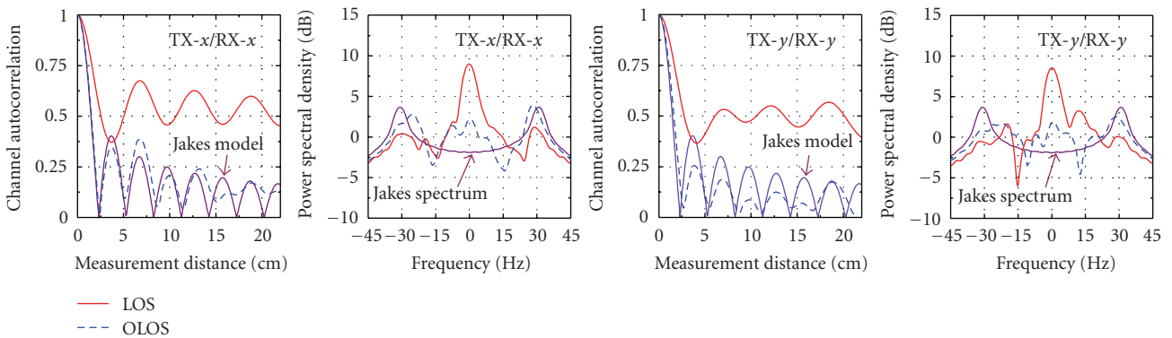
FIGURE 13: Channel autocorrelation and Doppler spectrum for f_D = 31 Hz of 2 \times 2 MIMO channels.
