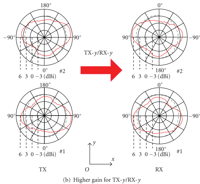
FIGURE 6: Antenna gain toward the direct wave for the case of AS = 0.5λ.
