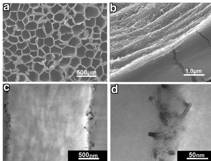
Figure 1. MWCNT-coated sponge. (a) SEM image of MWCNT-coated sponge. (b) SEM image of a cross section. (c) TEM image of a cross section. (d) High magnification of c.
