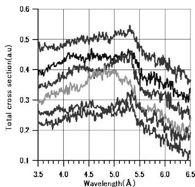
Fig.1 Examples of total cross-section depending on the position in fresh slow cooling LBE.
