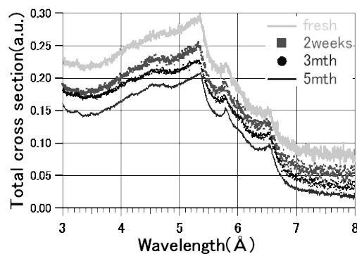
Fig.4 Changes of total cross-sections of rapid cooling LBE.
