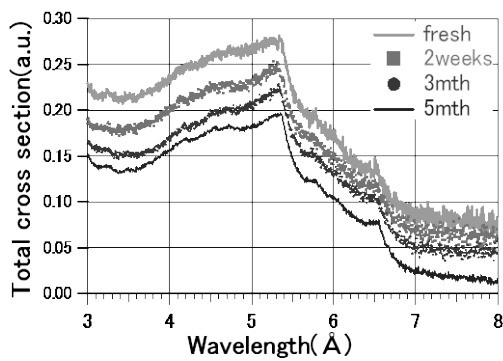
Fig.3 Changes of total cross-sections of slow cooling LBE.
