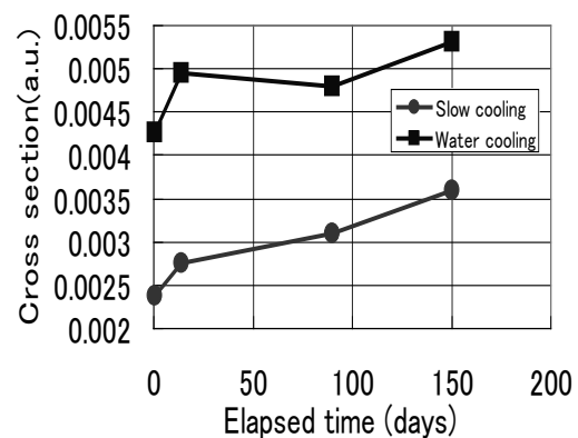
Fig.6 Time dependent cross-section change of the Bragg edge of Bi(012).
