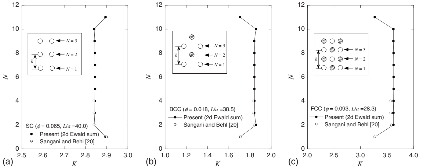
FIG. 3. Drag force acting on a dense particle layer for (a) SC array, (b) BCC array, and (c) FCC array (drag coefficient K=F/6\pi\mu aU ).
