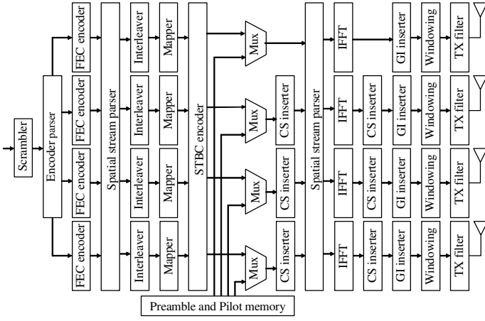
Fig. 1. Proposed Transmitter.
