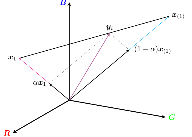
Fig. 2: Construction of the filter output as a weighted mean of the central pixel \mathbf{x}_1 and the vector median \mathbf{x}_{(1)} .
