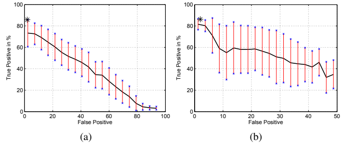
Fig. 8. ROC-curve for detecting the crucial (a) red and (b) green traffic light
