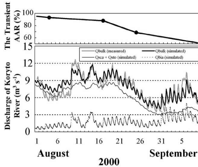
Fig. 5 Measured and simulated discharge of Koryto River and the variation in the transient accumulation area ratio (AAR) in the summer of 2000. Thick grey line and thick black line indicate measured and simulated bulk meltwater discharge. Thin line and dotted line indicate the component of meltwater from the snow-covered area plus stored water within the glacier, and the component of meltwater from bare ice area.
