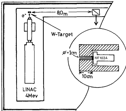
Fig. 1. Experimental arrangement
