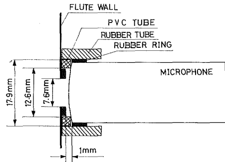
Fig. 8. A fitting of a condenser microphone to a finger hole of the flute.
