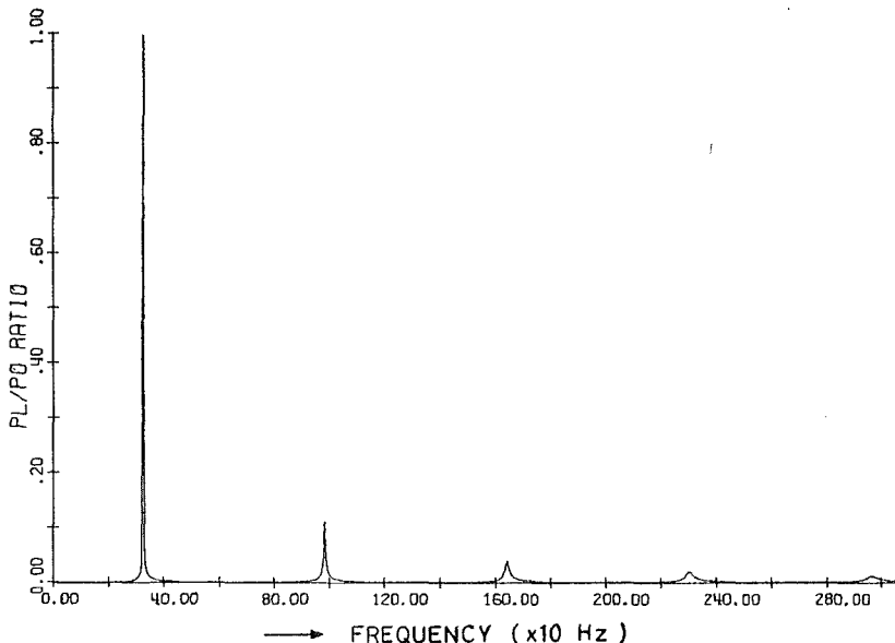
Fig. 3. Frequency response p_i/p_o(\omega) of a closed tube, calculated from the values: radius a=0.80 cm, length l=25.0 cm, at temperature 10^\circ\text{C} .
