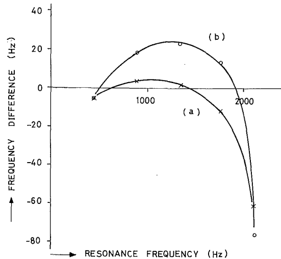
Fig. 13. Frequencies of the higher harmonics differed from the integral multiples of the fundamental frequency of the flute. Curve (a): frequency difference when the mouth hole was partially covered. Curve (b): frequency difference with this coverage removed. Sound source was placed at the mouth hole and the microphone was in place of the stopper. Some finger holes were closed according to A-fingering (440 and 880 Hz by overblowing).
