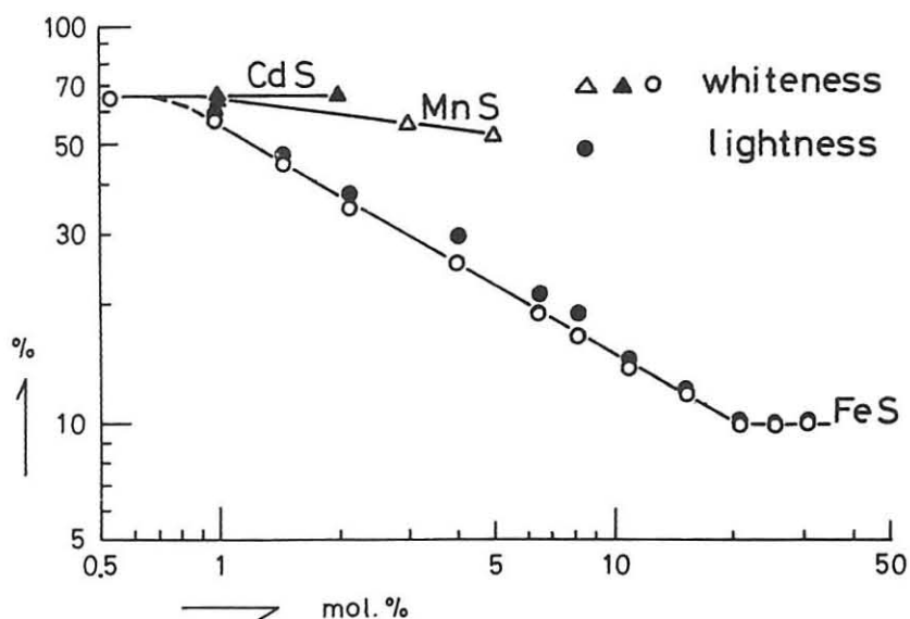
Text-Fig. 7 The relation between trichromatic subordinate properties and chemical components in sphalerite substituting for Zn ion on crystal structure.
