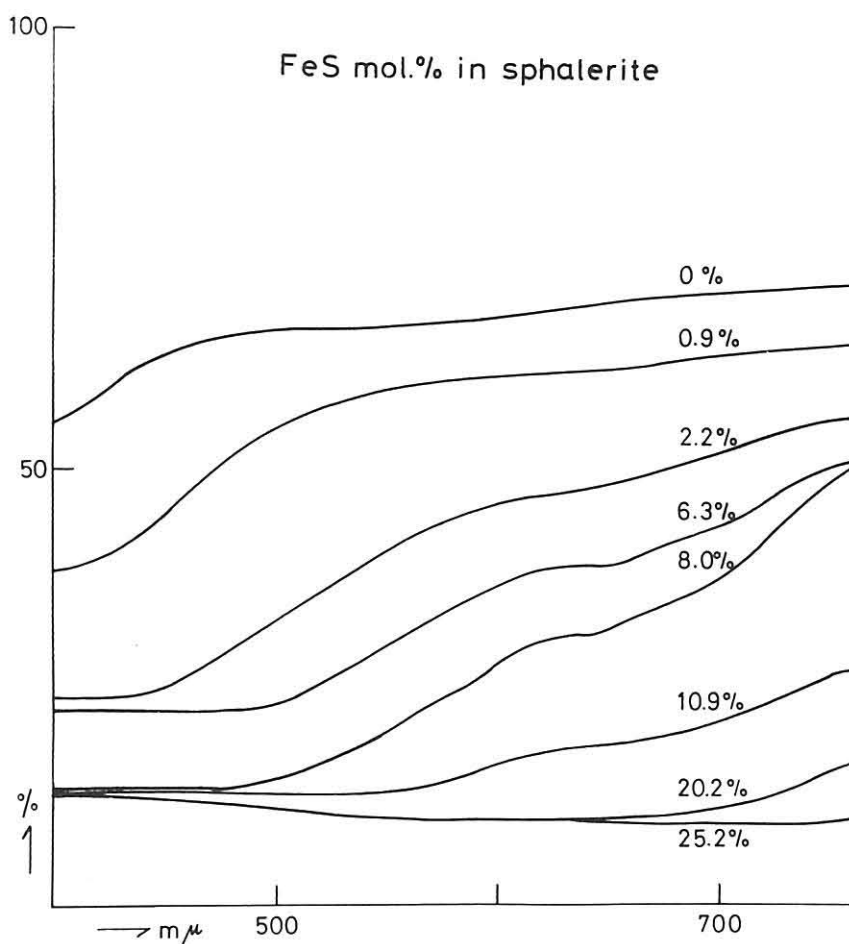
Text-Fig. 1 Spectroscopic reflectivity of sphalerite in which the Fe ion substitutes for position of Zn ion in crystal structure. Numbers above each curve show FeS mol. % in sphalerite.
