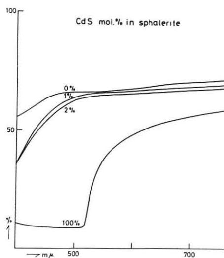
Text-Fig. 4 (Right) Spectroscopic reflectivity of sphalerite in which the Cd ion substitutes for Zn ion. Numbers above each curve show CdS mol. % in sphalerite. See Text-Fig. 1 for abscissa and ordinate.
