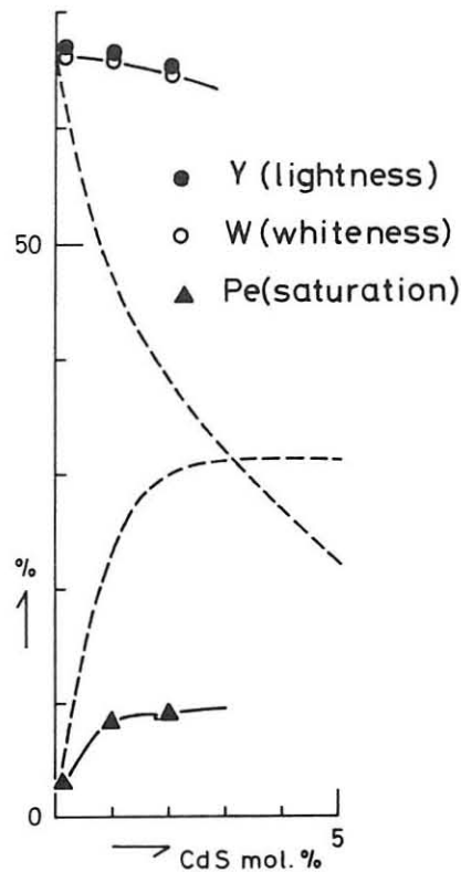
Text-Fig. 6 (Right) Trichromatic specification diagram of sphalerite in ZnS-CdS solid solution system.
