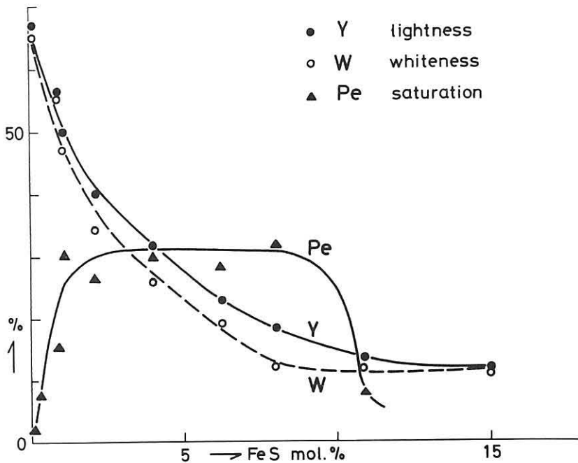
Text-Fig. 2 Trichromatic specification diagram of sphalerite in ZnS-FeS solid solution system. The lightness, whiteness, and saturation in colour are shown in percentage.
