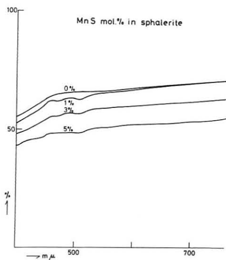
Text-Fig. 3 (Left) Spectroscopic reflectivity of sphalerite in which the Mn ion substitutes for Zn ion. Numbers above each curve show MnS mol. % in sphalerite. See Text-fig. 1 for abscissa and ordinate.
