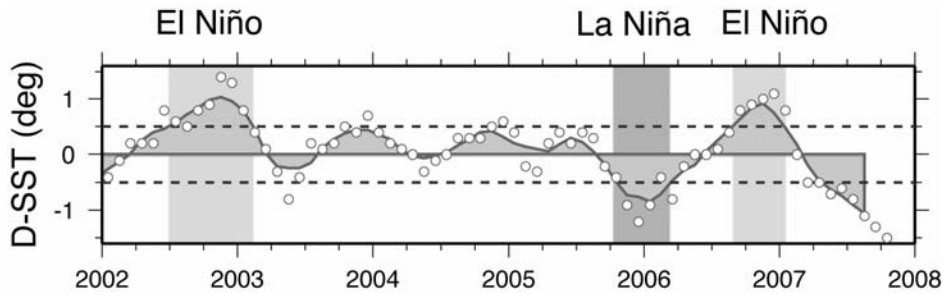
Fig.2. Monthly differences (open circles) between the SST in the El Niño monitoring area and the reference temperature, from the Japan Meteorological Agency website ( www.jma.go.jp ). The black curve shows the 5 months moving average. In an El Niño/La Niña episode, the black curve stays above/below the \pm 0.5 degree level (dashed lines) for a half year or more.
