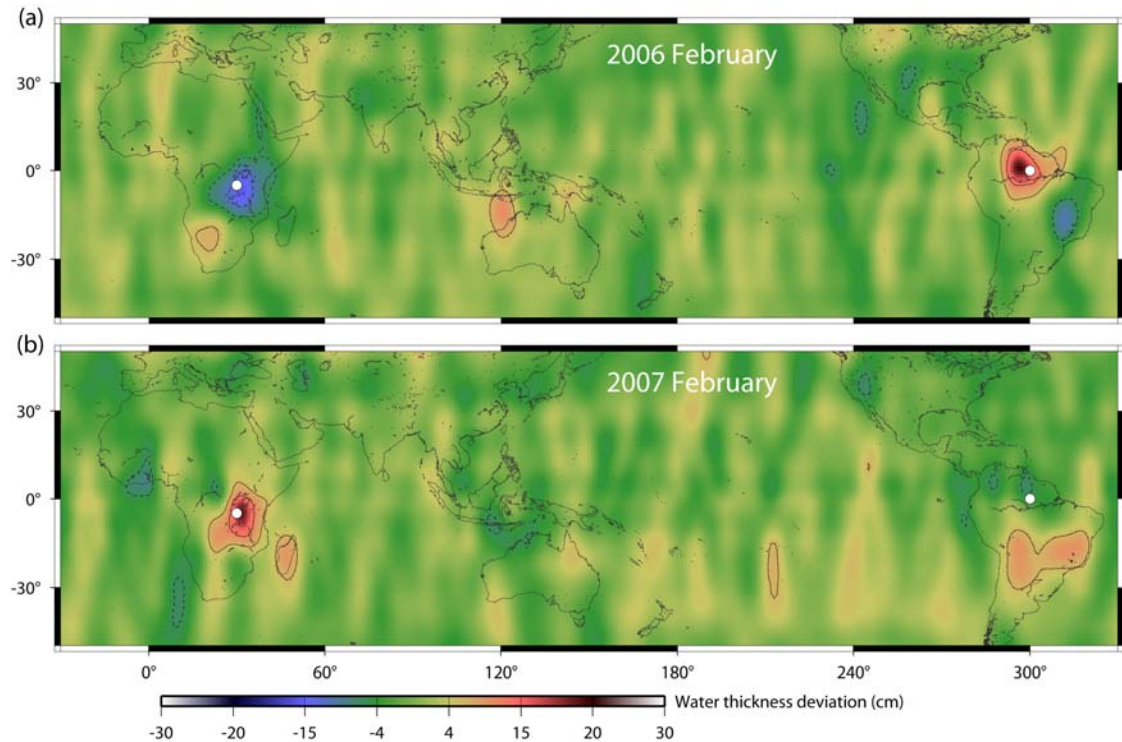
Fig. 4. Gravity deviations from standard seasonal curves converted into water thickness deviations in February 2006 (a) and February 2007 (b), which represents the recent La Niña and El Niño episodes, respectively. Contours show \pm 6 and \pm 12 cm (broken contours are negative). The \pm 6 cm contours approximately correspond to the 2\sigma error inferred by the time series analysis (Fig.3). The two white circles show points in Tanzania and Brazil, whose time series are plotted in Fig. 3. A Gaussian filter with the averaging radius of 500 km has been applied. Stripes striking north-south are apparent signals coming from correlated errors [21].
