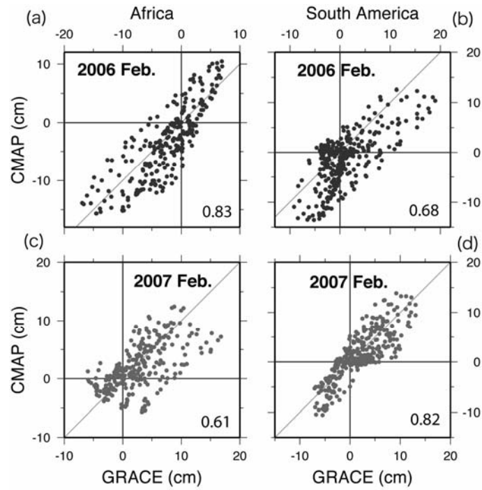
Fig.8 Correlation between water thickness deviations by GRACE and CMAP in 2006 (a,b) and 2007 (c,d) February at 2.5 x 2.5 degree grid points in the African (a,c) (latitude 30S-5N, longitude 10E-55E) and South American (b,d) (latitude 35S-10N, longitude 285E-325E) continents. Numbers in the figure indicates the correlation coefficients.
