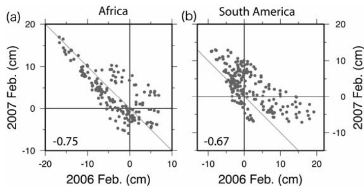
Fig.5 Correlation between water thickness deviations in 2006 and 2007 February at 2.5 \times 2.5 degree grid points in the African (a) (latitude 30S-5N, longitude 10E-55E) and South American (b) (latitude 35S-10N, longitude 285E-325E) continents. Numbers in the figure indicates the correlation coefficients.
