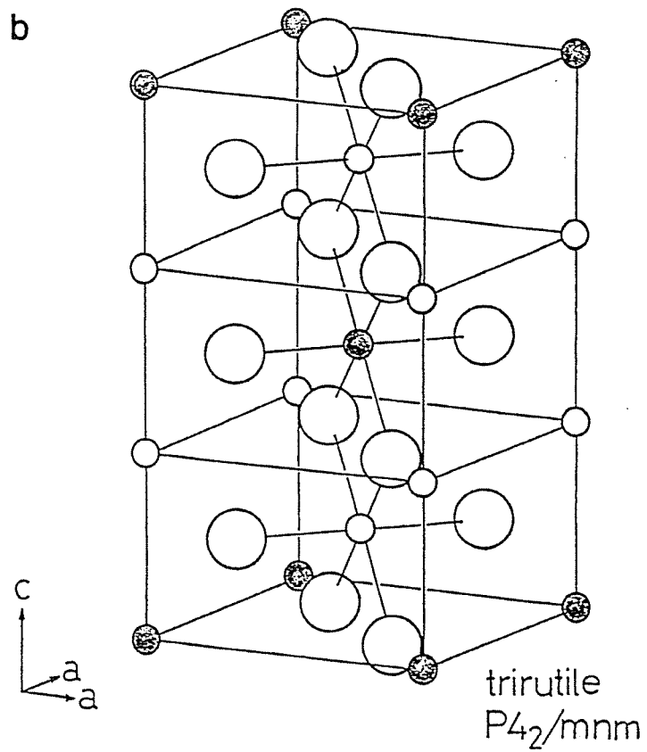
Fig. 7. Crystal structures of rutile (a) and trirutile (b). Large open circles represent oxide ions and small circles represent cations.
