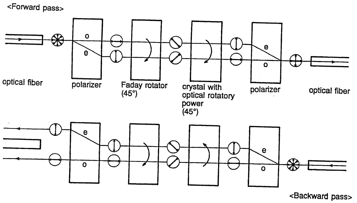
Fig. 5. Principle of an optical isolator using parallel plates as polarizers.
