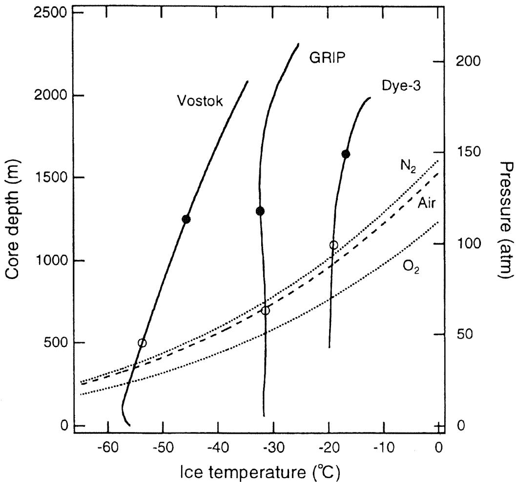
Figure 1: Relationship between temperature and dissociation pressures of N 2 -, O 2 -, and air- (N 2 /O 2 = 3.7) clathrate hydrates. The solid lines are the depth profiles of the ice temperatures of Vostok, GRIP, and Dye-3 ice cores. The open and solid circles show the depths below which clathrate hydrate crystals are observed and below which air-bubbles are not observed, respectively.
