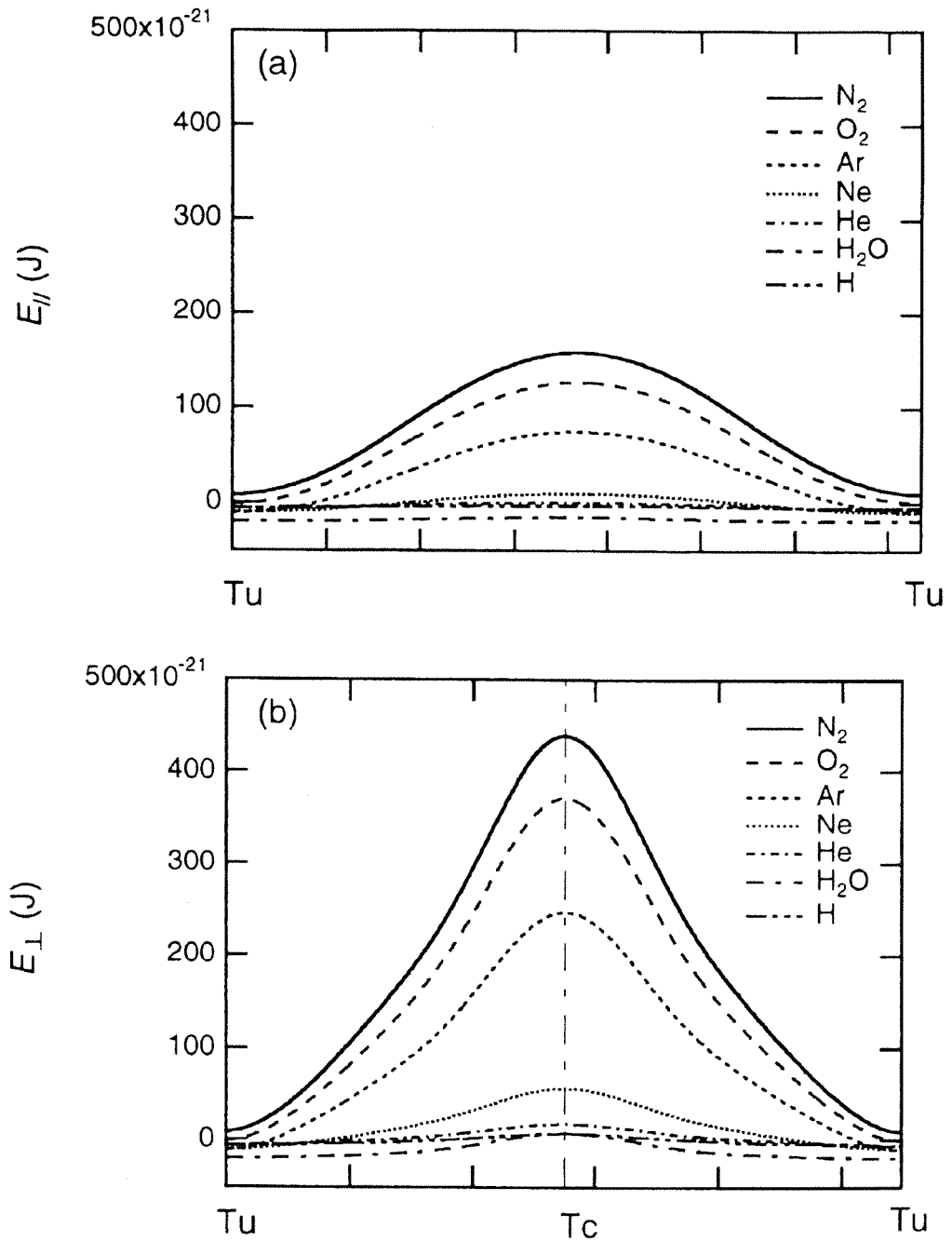
Figure 9: The intermolecular interaction energies between a gas molecule and surrounding water molecules. (a) The gas molecules jump in ice Ih parallel to the c-axis (i.e., Tu \rightarrow Tu ). (b) The gas molecules jump in ice Ih perpendicular to the c-axis (i.e., Tu \rightarrow Tc \rightarrow Tu ).
