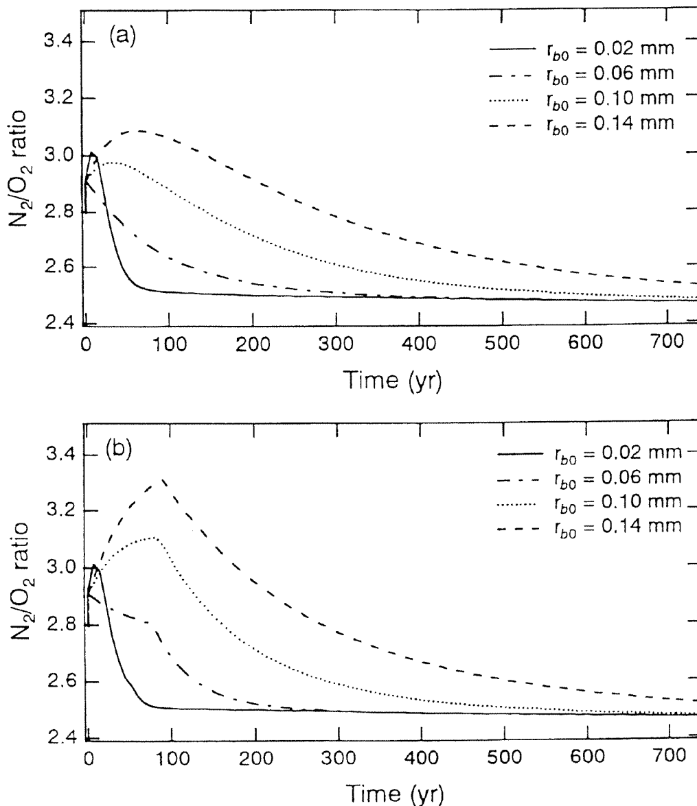
Figure 14: Temporal variation of the N_2/O_2 ratio in a clathrate hydrate at the beginning of the transition zone of the GRIP ice core (800 m in depth). (a) The growth process of type A. (b) The growth process of type B. r_{b0} is the radius of the initial air-bubble.
