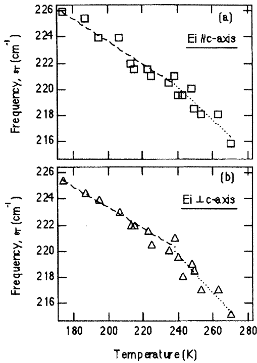
Figure 13: The T dependence of the frequency of translational lattice vibrations in DF ice observed by Raman spectroscopy of the c -axis parallel, (a), and perpendicular, (b), to the electric field [55].
