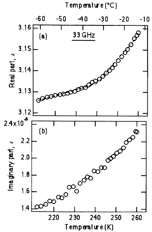
Figure 14: Temperature dependence of permittivities of DF ice core at 33 GHz [55]. (a) real part, \varepsilon' , (b) imaginary part, \varepsilon'' .
