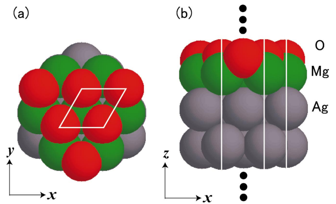
FIG. 2. (Color) Top (a) and side (b) views of the atomic configuration considered in the present study. The unit cell is indicated in white.
