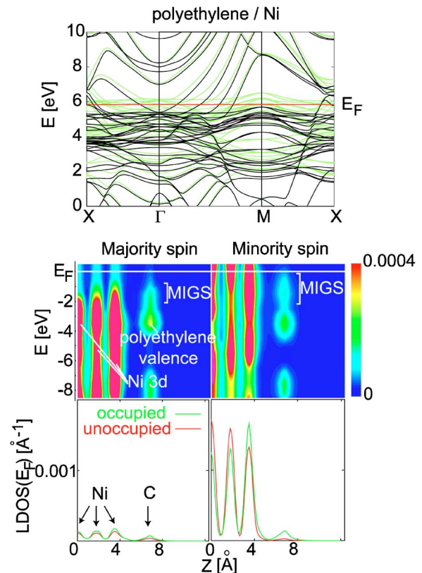
FIG. 3. (Color online) A plot similar to Fig. 2 for 1 ML polyethylene/Ni(001), where the spin density functional theory is adopted. Green (black) lines in the band structure represent the majority (minority) spin.
