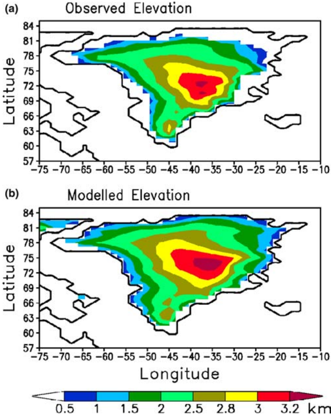
Figure 3: Surface elevation of the Greenland ice sheet in kilometres: a observed after Letréguilly et al. (1991), and b from a steady-state simulation with the fully coupled model.
