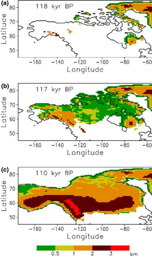
Figure 6: Surface elevation of the inland ice in North America in AOV1 at a 118 kyr BP, b 117 kyr BP and c 110 kyr BP. The elevation is given in kilometres.
