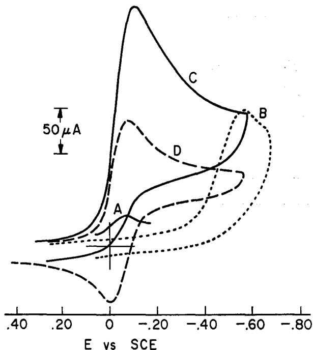
Fig. 3. Cyclic voltammograms at Tokai glassy carbon electrode. . . A: 2 \times 10^{-4} M Fe(III) TMPyP, B: only O_2 (air-saturated), C: mixture of 2 \times 10^{-4} M Fe(III) TMPyP and O_2 (air-saturated), and D: 10^{-8} M Fe(III) TMPyP, no O_2 . All solutions contain 0.1 N H_2SO_4 . Scan rate: 0.11 V/sec.
